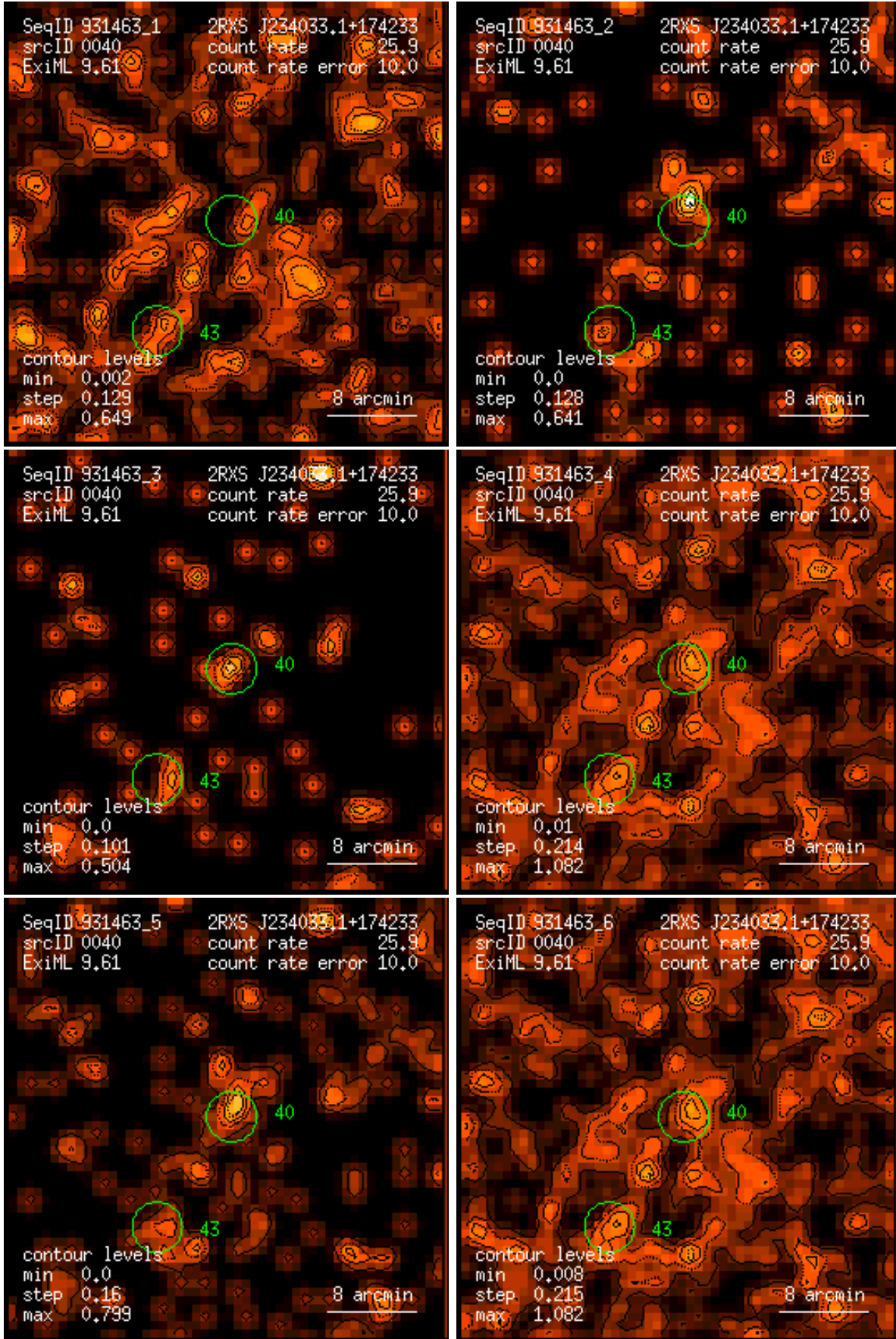
Figure 40: RASS 931463: detection 0040: band rate images, Gaussian filter: (1) PSPC channels 11 – 41, (2) 52 – 90, (3) 91 – 201, (4) 11 – 235, (5) 52 – 201, (6) 11 – 201. Broad band rates in counts/ks. Band rate contour levels in counts/ks/arcmin 2 .
