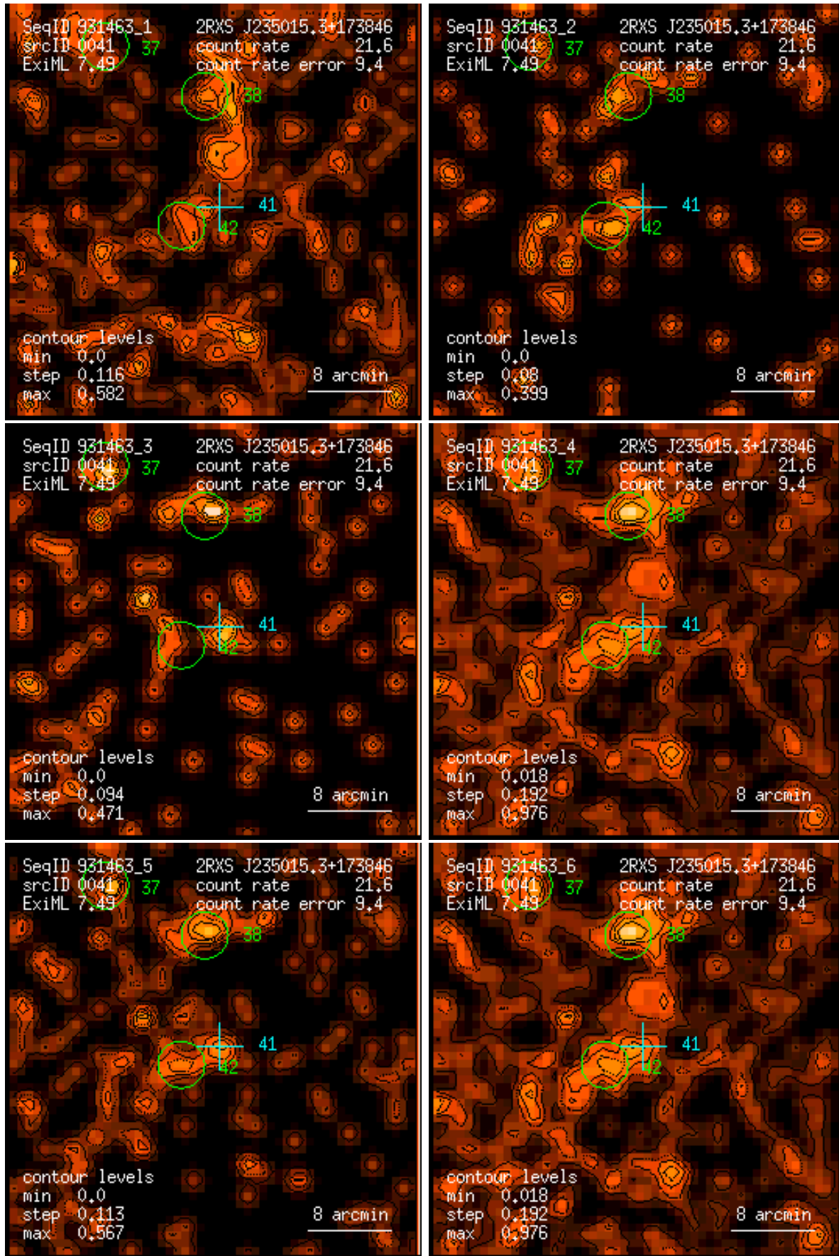
Figure 41: RASS 931463: detection 0041: band rate images, Gaussian filter: (1) PSPC channels 11 – 41, (2) 52 – 90, (3) 91 – 201, (4) 11 – 235, (5) 52 – 201, (6) 11 – 201. Broad band rates in counts/ks. Band rate contour levels in counts/ks/arcmin 2 .
