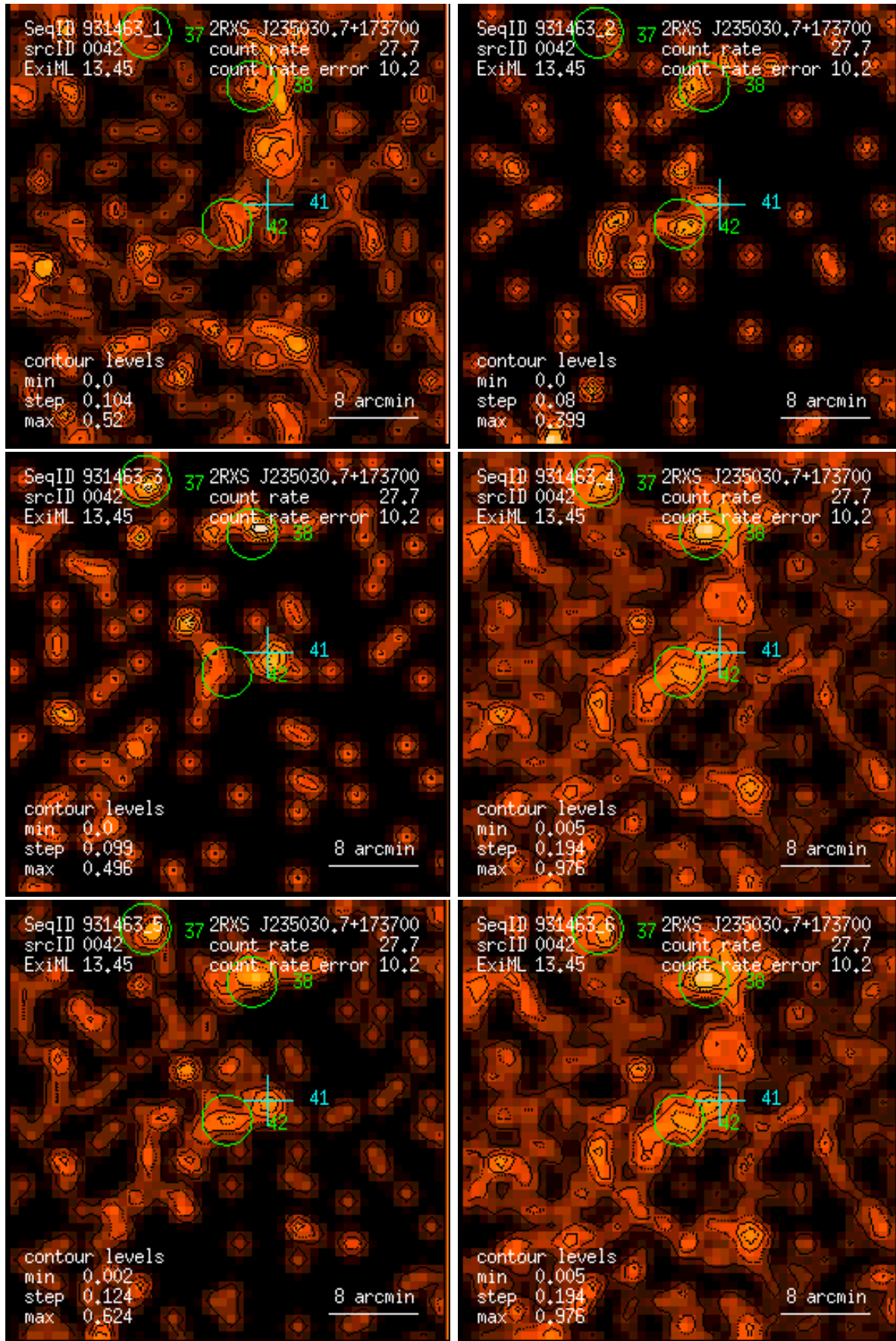
Figure 42: RASS 931463: detection 0042: band rate images, Gaussian filter: (1) PSPC channels 11 – 41, (2) 52 – 90, (3) 91 – 201, (4) 11 – 235, (5) 52 – 201, (6) 11 – 201. Broad band rates in counts/ks. Band rate contour levels in counts/ks/arcmin 2 .
