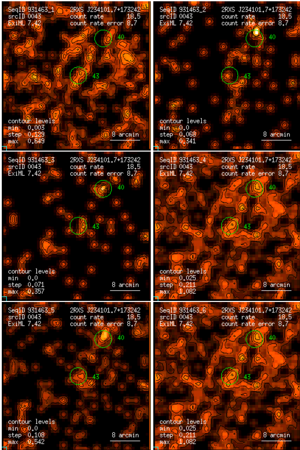
Figure 43: RASS 931463: detection 0043: band rate images, Gaussian filter: (1) PSPC channels 11 – 41, (2) 52 – 90, (3) 91 – 201, (4) 11 – 235, (5) 52 – 201, (6) 11 – 201. Broad band rates in counts/ks. Band rate contour levels in counts/ks/arcmin 2 .
