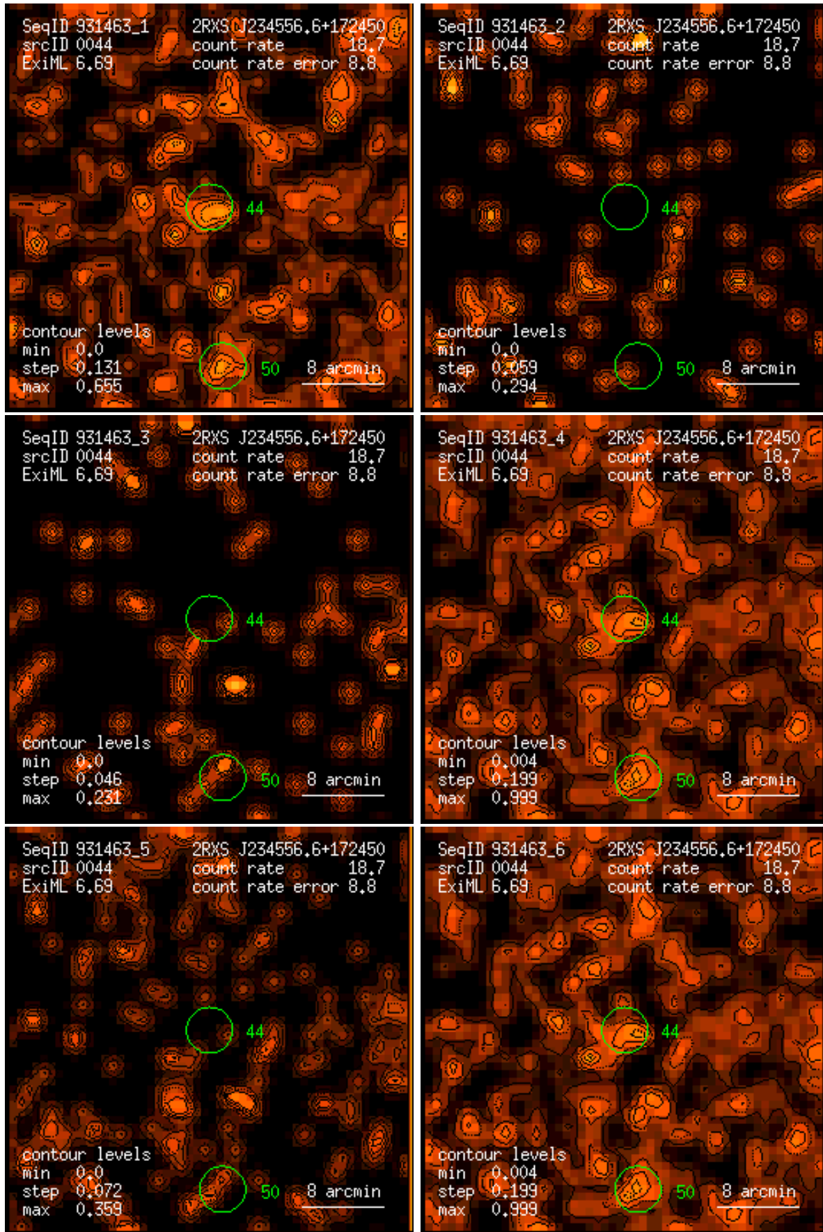
Figure 44: RASS 931463: detection 0044: band rate images, Gaussian filter: (1) PSPC channels 11 – 41, (2) 52 – 90, (3) 91 – 201, (4) 11 – 235, (5) 52 – 201, (6) 11 – 201. Broad band rates in counts/ks. Band rate contour levels in counts/ks/arcmin 2 .
