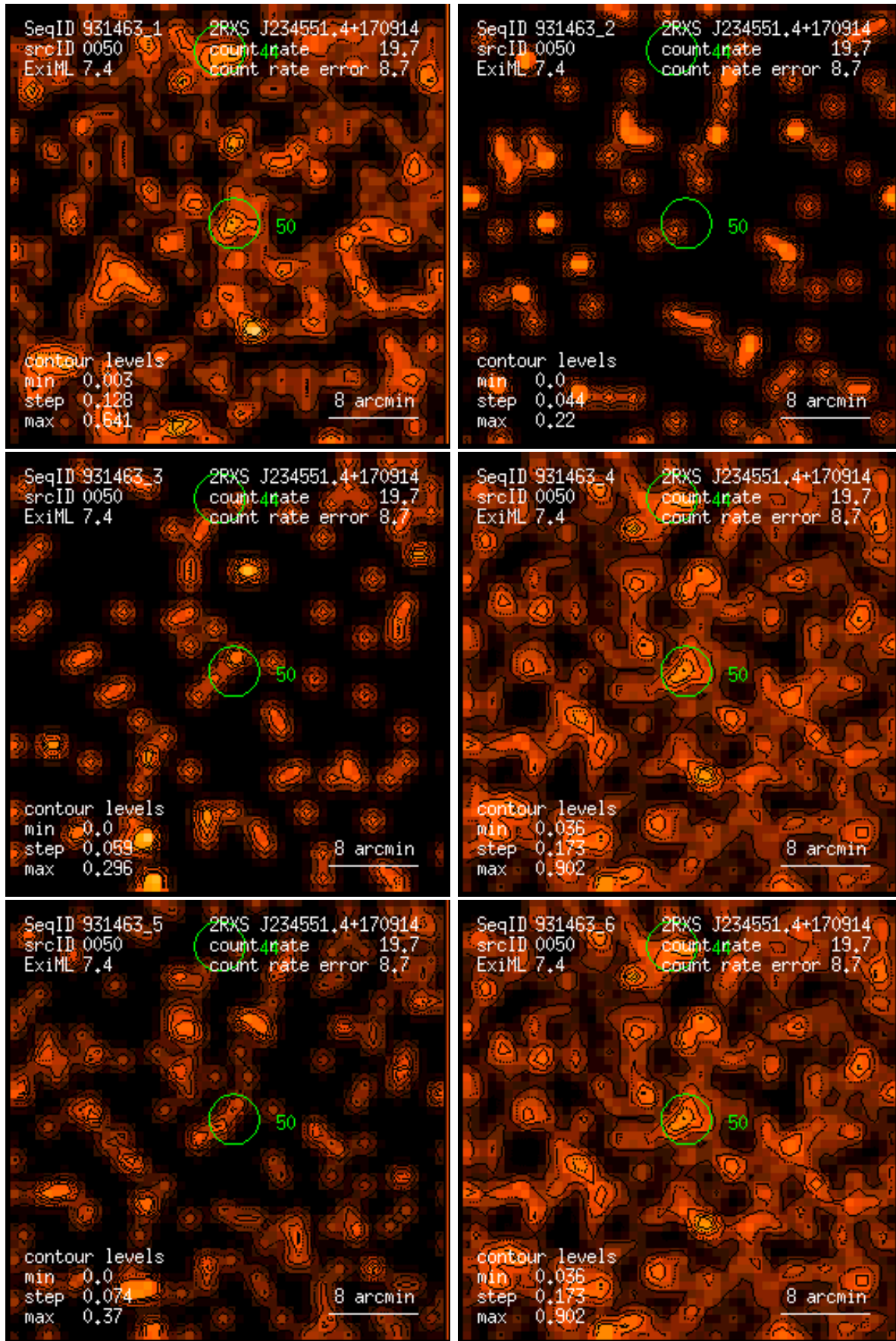
Figure 50: RASS 931463: detection 0050: band rate images, Gaussian filter: (1) PSPC channels 11 – 41, (2) 52 – 90, (3) 91 – 201, (4) 11 – 235, (5) 52 – 201, (6) 11 – 201. Broad band rates in counts/ks. Band rate contour levels in counts/ks/arcmin 2 .
