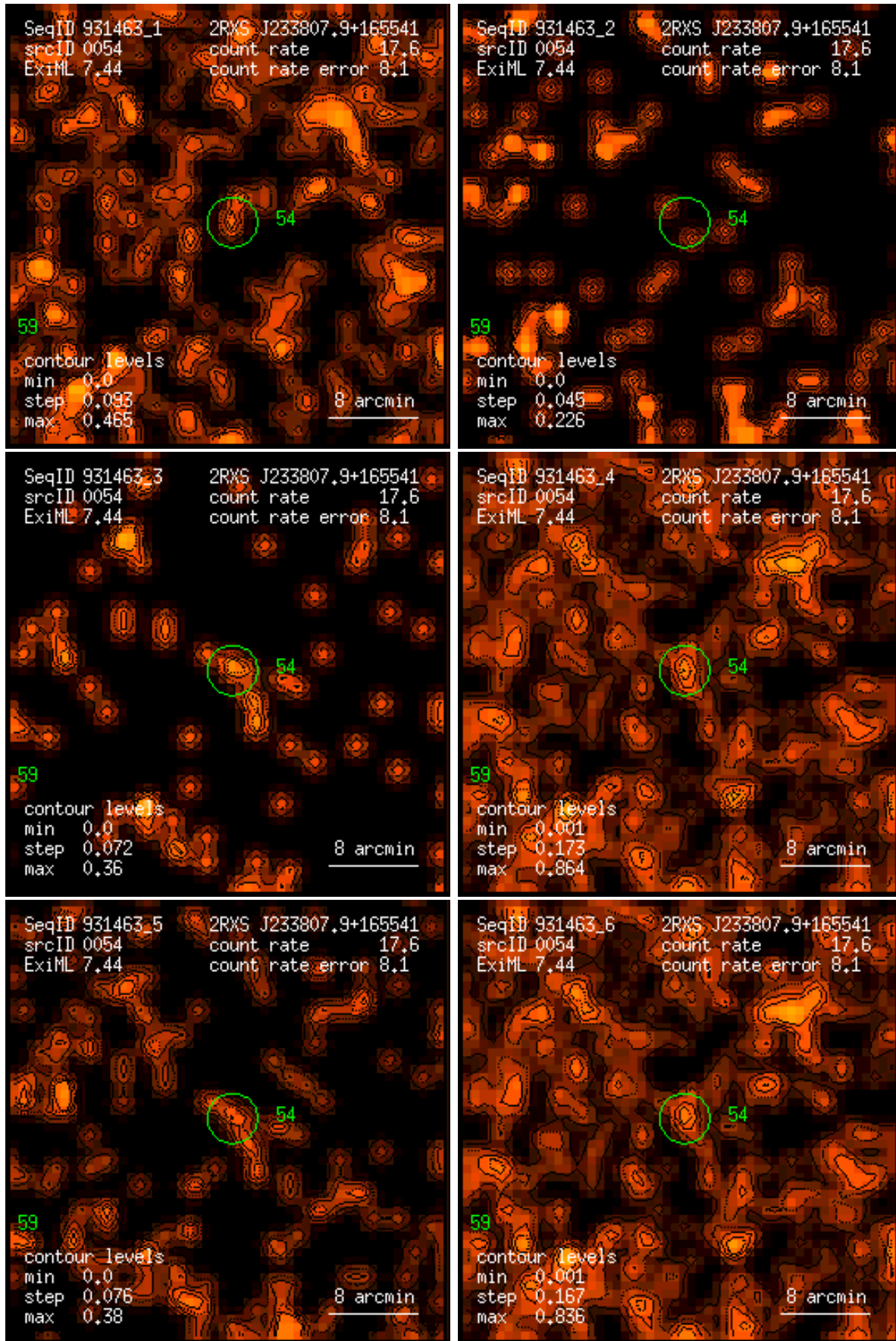
Figure 54: RASS 931463: detection 0054: band rate images, Gaussian filter: (1) PSPC channels 11 – 41, (2) 52 – 90, (3) 91 – 201, (4) 11 – 235, (5) 52 – 201, (6) 11 – 201. Broad band rates in counts/ks. Band rate contour levels in counts/ks/arcmin 2 .
