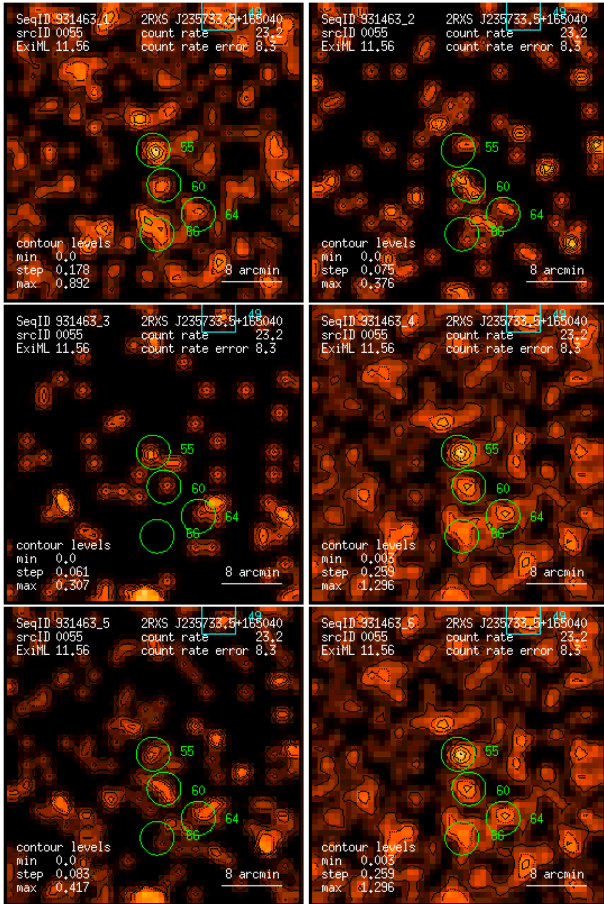
Figure 55: RASS 931463: detection 0055: band rate images, Gaussian filter: (1) PSPC channels 11 – 41, (2) 52 – 90, (3) 91 – 201, (4) 11 – 235, (5) 52 – 201, (6) 11 – 201. Broad band rates in counts/ks. Band rate contour levels in counts/ks/arcmin 2 .
