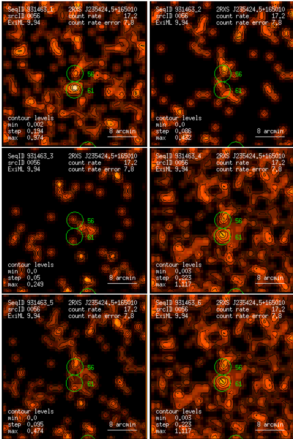
Figure 56: RASS 931463: detection 0056: band rate images, Gaussian filter: (1) PSPC channels 11 – 41, (2) 52 – 90, (3) 91 – 201, (4) 11 – 235, (5) 52 – 201, (6) 11 – 201. Broad band rates in counts/ks. Band rate contour levels in counts/ks/arcmin 2 .
