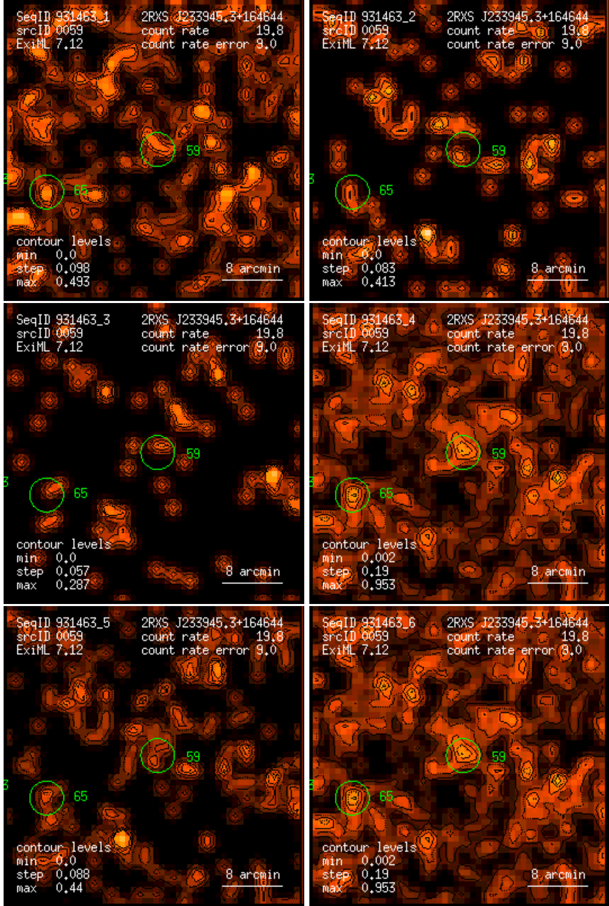
Figure 59: RASS 931463: detection 0059: band rate images, Gaussian filter: (1) PSPC channels 11 – 41, (2) 52 – 90, (3) 91 – 201, (4) 11 – 235, (5) 52 – 201, (6) 11 – 201. Broad band rates in counts/ks. Band rate contour levels in counts/ks/arcmin 2 .
