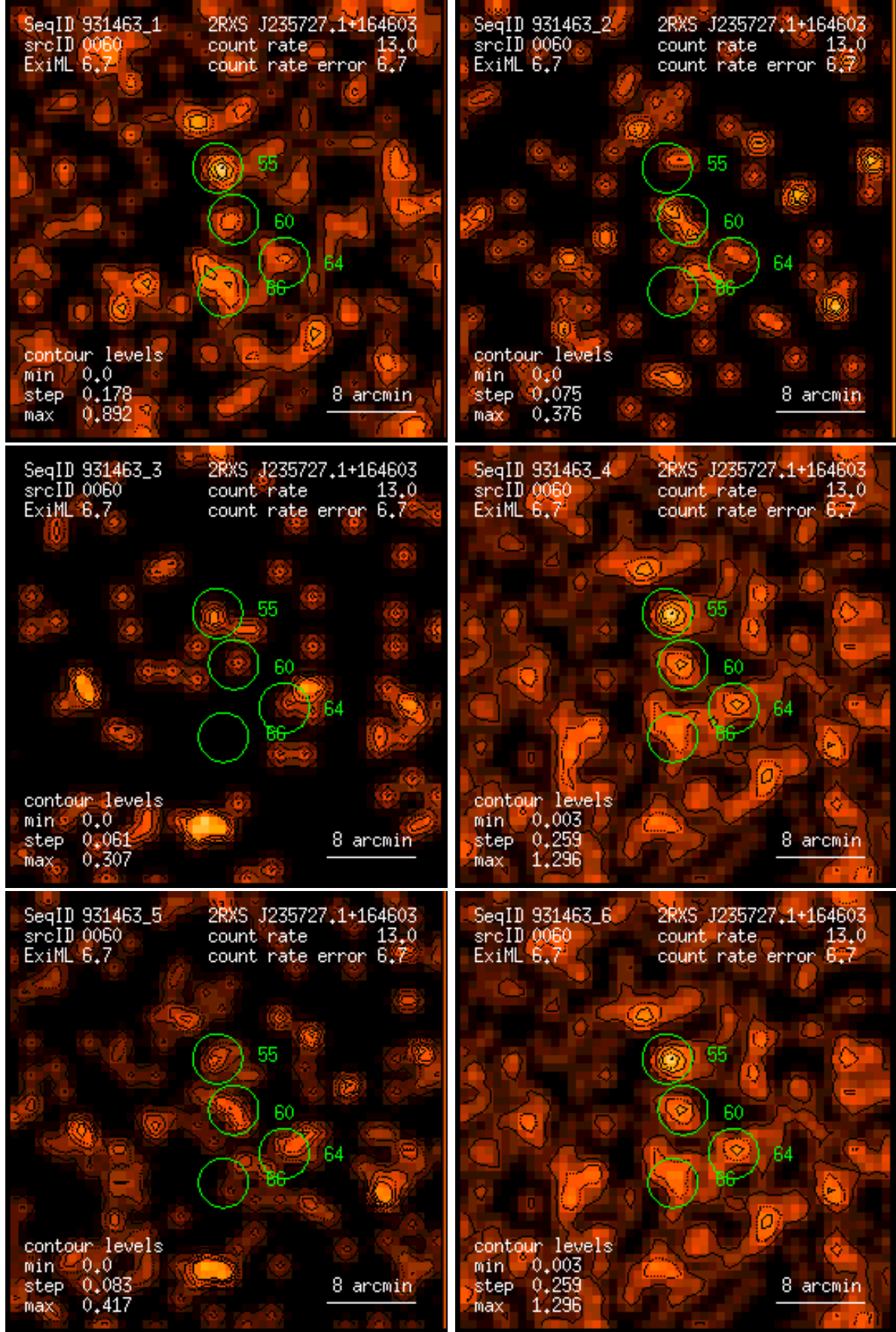
Figure 60: RASS 931463: detection 0060: band rate images, Gaussian filter: (1) PSPC channels 11 – 41, (2) 52 – 90, (3) 91 – 201, (4) 11 – 235, (5) 52 – 201, (6) 11 – 201. Broad band rates in counts/ks. Band rate contour levels in counts/ks/arcmin 2 .
