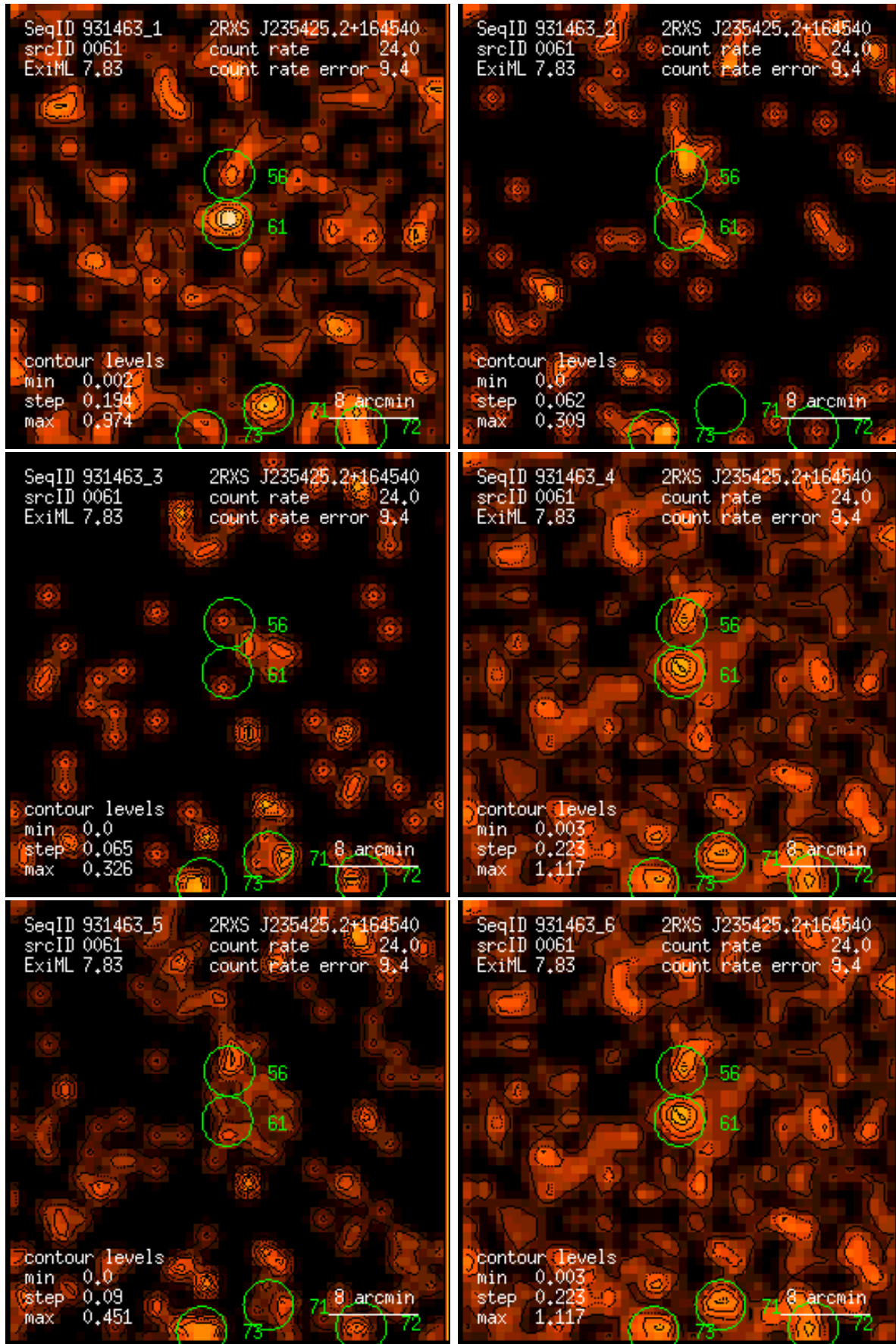
Figure 61: RASS 931463: detection 0061: band rate images, Gaussian filter: (1) PSPC channels 11 – 41, (2) 52 – 90, (3) 91 – 201, (4) 11 – 235, (5) 52 – 201, (6) 11 – 201. Broad band rates in counts/ks. Band rate contour levels in counts/ks/arcmin 2 .
