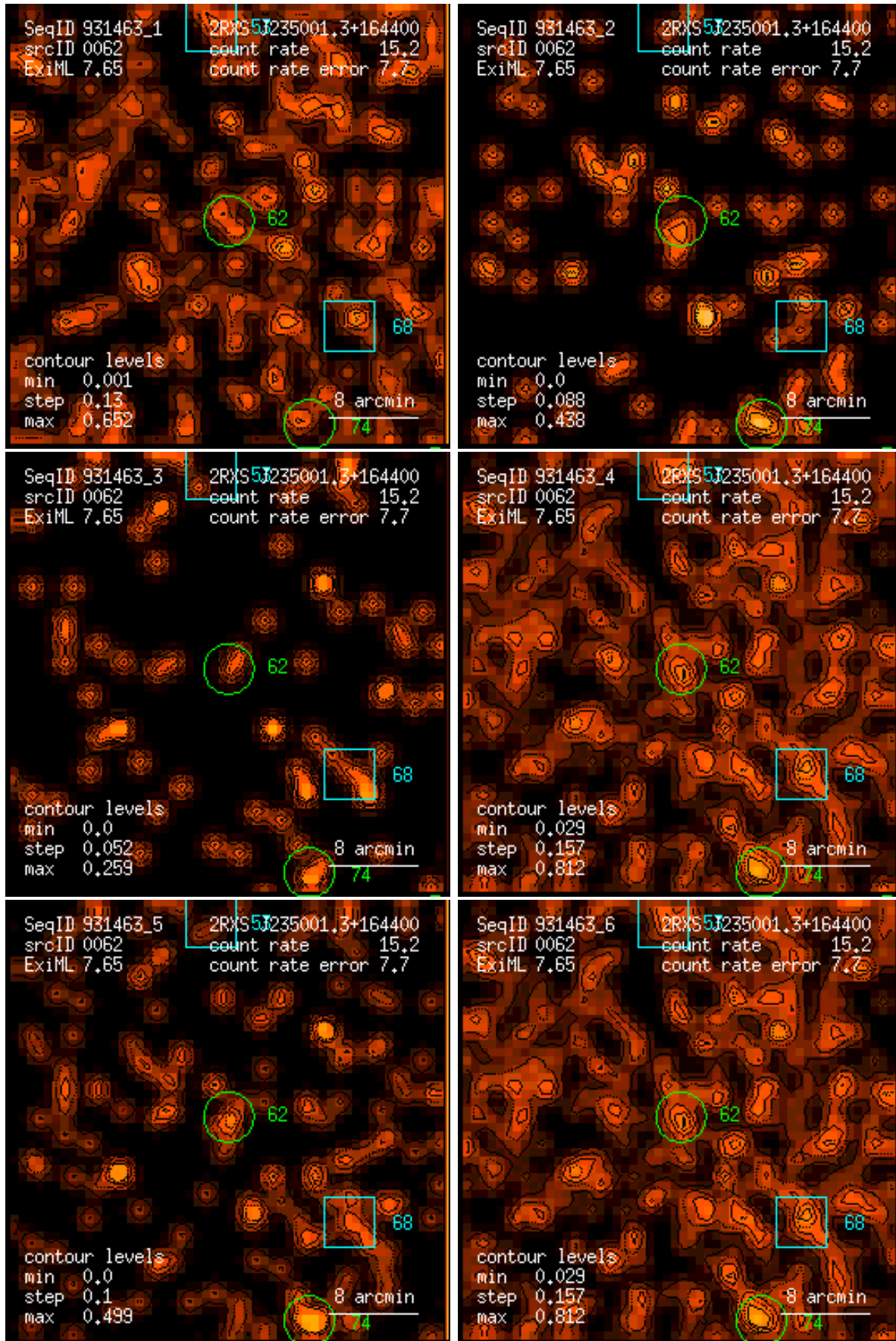
Figure 62: RASS 931463: detection 0062: band rate images, Gaussian filter: (1) PSPC channels 11 – 41, (2) 52 – 90, (3) 91 – 201, (4) 11 – 235, (5) 52 – 201, (6) 11 – 201. Broad band rates in counts/ks. Band rate contour levels in counts/ks/arcmin 2 .
