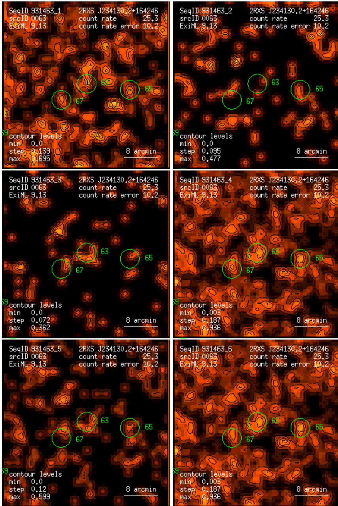
Figure 63: RASS 931463: detection 0063: band rate images, Gaussian filter: (1) PSPC channels 11 – 41, (2) 52 – 90, (3) 91 – 201, (4) 11 – 235, (5) 52 – 201, (6) 11 – 201. Broad band rates in counts/ks. Band rate contour levels in counts/ks/arcmin 2 .
