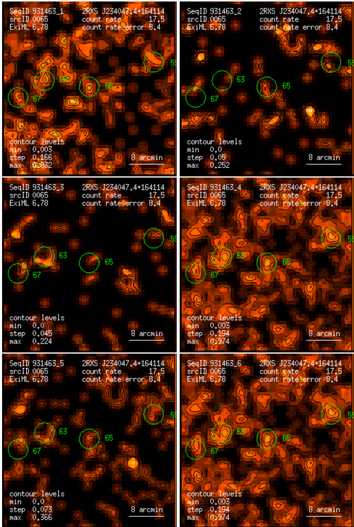
Figure 65: RASS 931463: detection 0065: band rate images, Gaussian filter: (1) PSPC channels 11 – 41, (2) 52 – 90, (3) 91 – 201, (4) 11 – 235, (5) 52 – 201, (6) 11 – 201. Broad band rates in counts/ks. Band rate contour levels in counts/ks/arcmin 2 .
