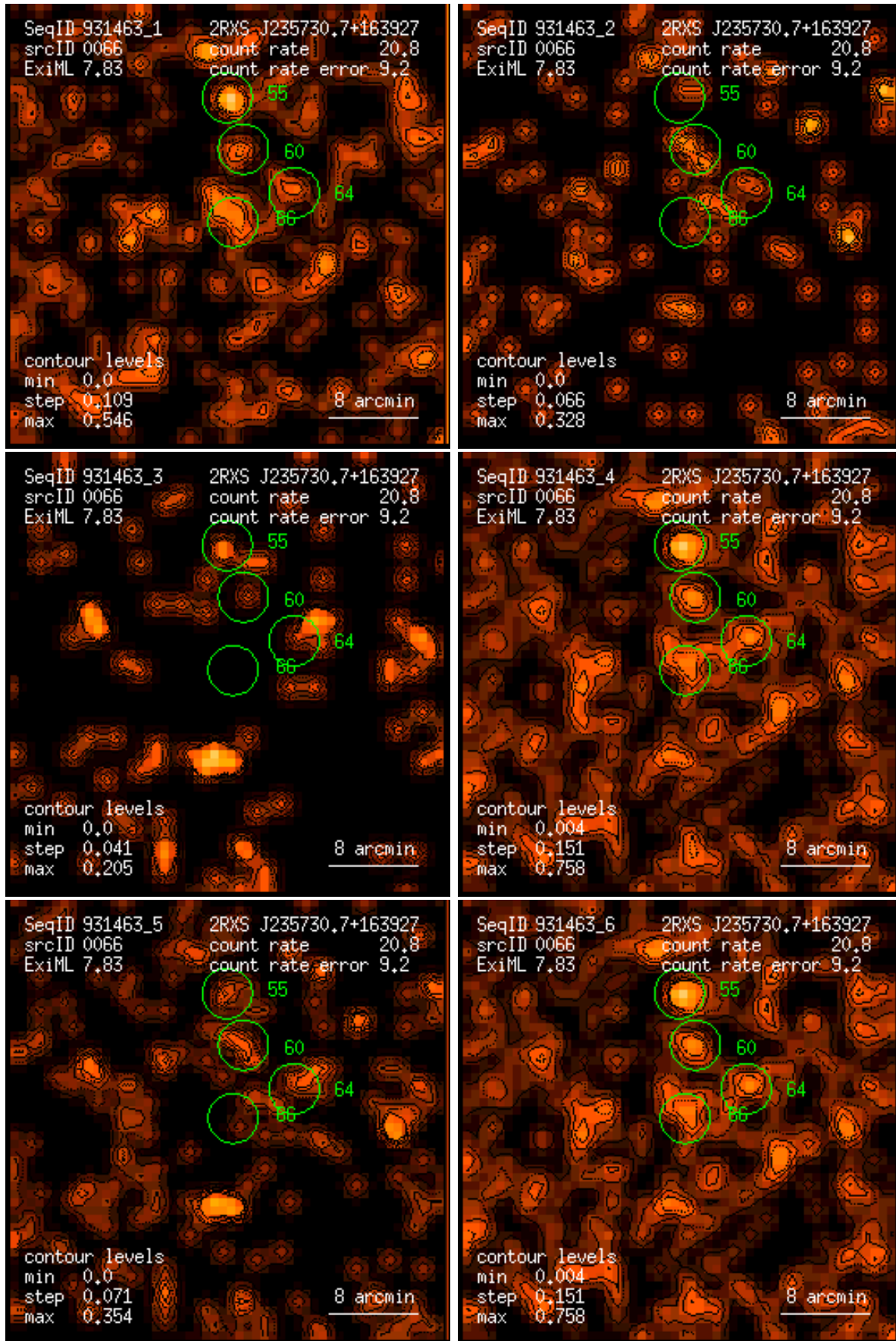
Figure 66: RASS 931463: detection 0066: band rate images, Gaussian filter: (1) PSPC channels 11 – 41, (2) 52 – 90, (3) 91 – 201, (4) 11 – 235, (5) 52 – 201, (6) 11 – 201. Broad band rates in counts/ks. Band rate contour levels in counts/ks/arcmin 2 .
