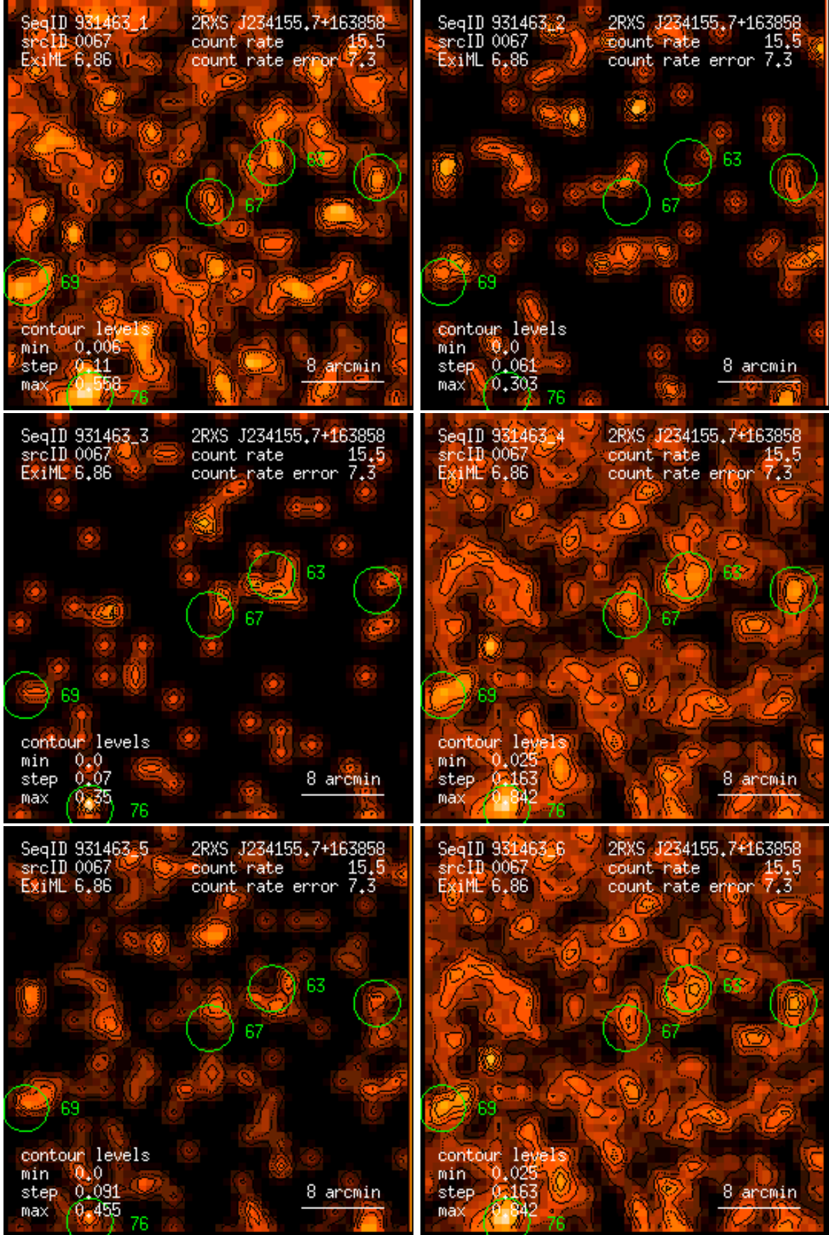
Figure 67: RASS 931463: detection 0067: band rate images, Gaussian filter: (1) PSPC channels 11 – 41, (2) 52 – 90, (3) 91 – 201, (4) 11 – 235, (5) 52 – 201, (6) 11 – 201. Broad band rates in counts/ks. Band rate contour levels in counts/ks/arcmin 2 .
