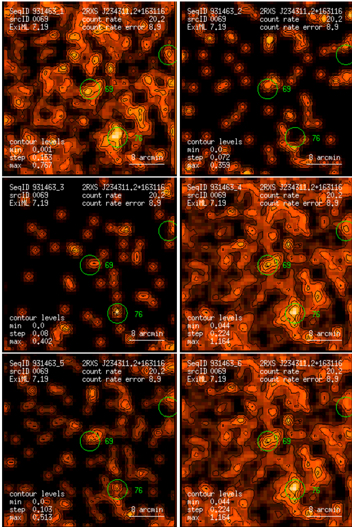
Figure 69: RASS 931463: detection 0069: band rate images, Gaussian filter: (1) PSPC channels 11 – 41, (2) 52 – 90, (3) 91 – 201, (4) 11 – 235, (5) 52 – 201, (6) 11 – 201. Broad band rates in counts/ks. Band rate contour levels in counts/ks/arcmin 2 .
