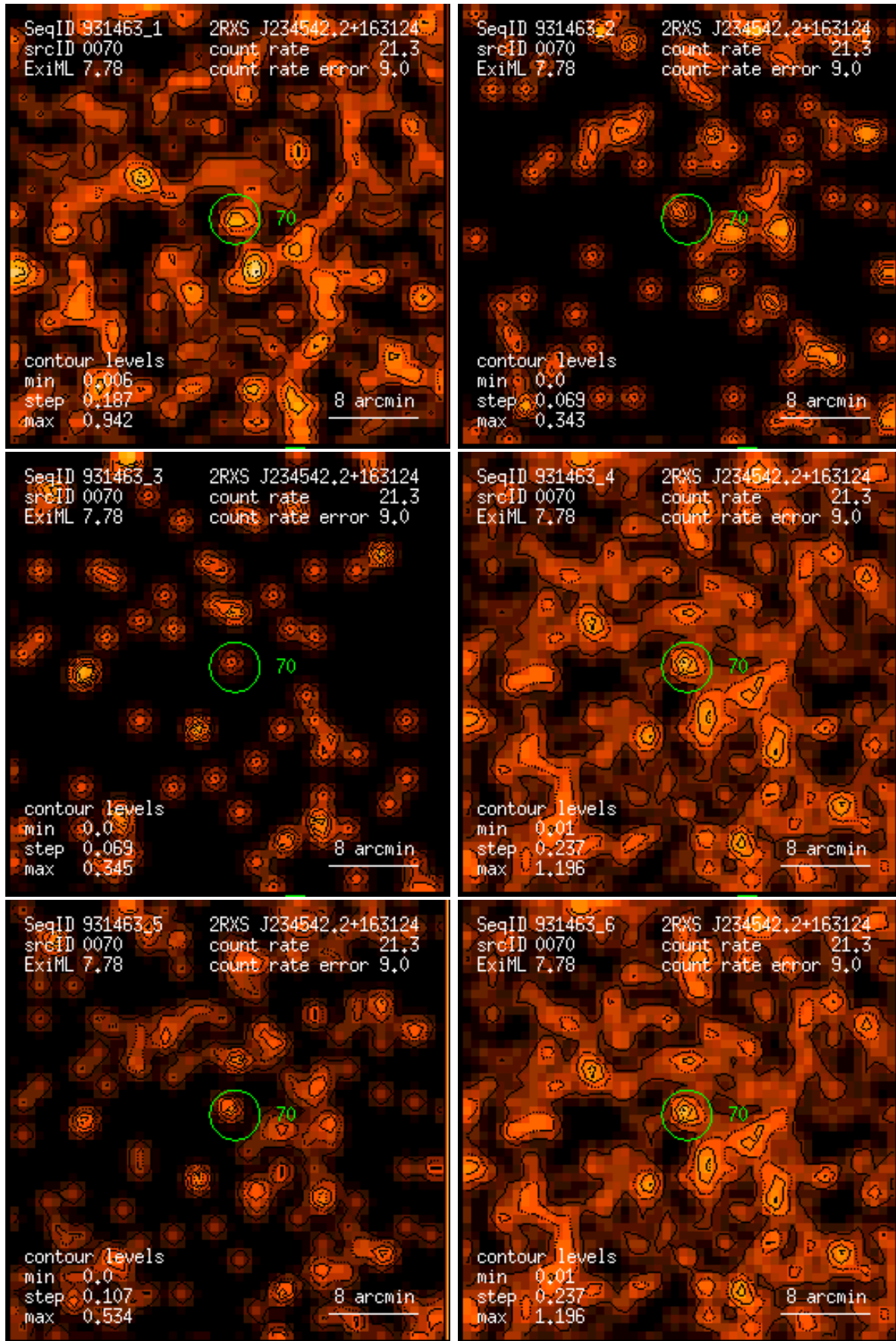
Figure 70: RASS 931463: detection 0070: band rate images, Gaussian filter: (1) PSPC channels 11 – 41, (2) 52 – 90, (3) 91 – 201, (4) 11 – 235, (5) 52 – 201, (6) 11 – 201. Broad band rates in counts/ks. Band rate contour levels in counts/ks/arcmin 2 .
