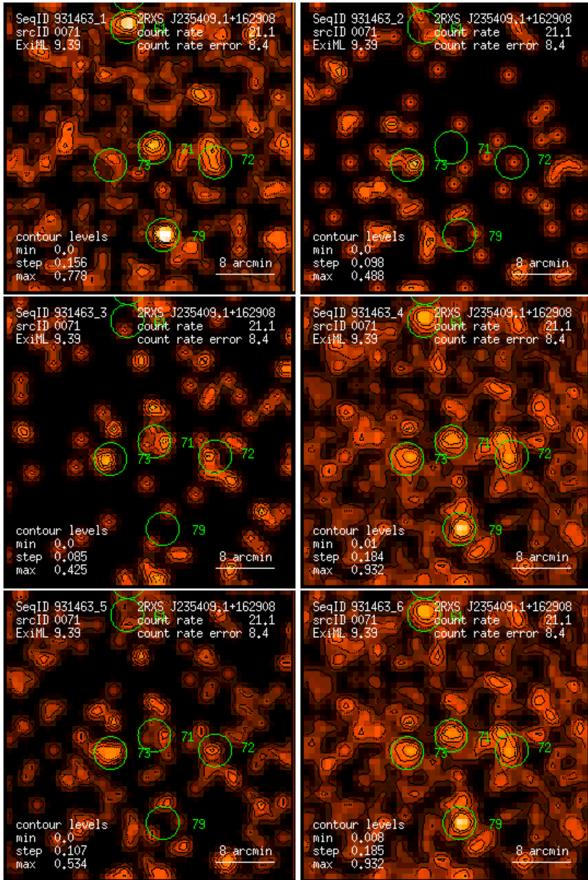
Figure 71: RASS 931463: detection 0071: band rate images, Gaussian filter: (1) PSPC channels 11 – 41, (2) 52 – 90, (3) 91 – 201, (4) 11 – 235, (5) 52 – 201, (6) 11 – 201. Broad band rates in counts/ks. Band rate contour levels in counts/ks/arcmin 2 .
