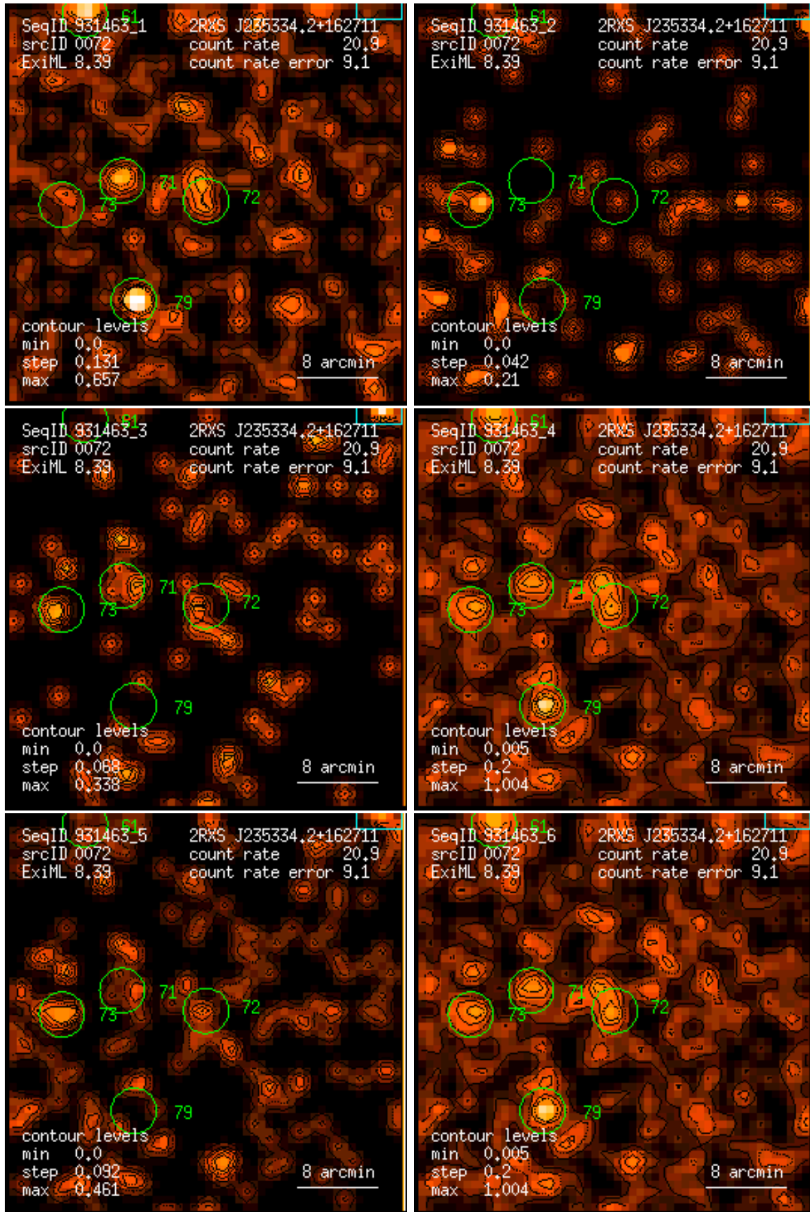
Figure 72: RASS 931463: detection 0072: band rate images, Gaussian filter: (1) PSPC channels 11 – 41, (2) 52 – 90, (3) 91 – 201, (4) 11 – 235, (5) 52 – 201, (6) 11 – 201. Broad band rates in counts/ks. Band rate contour levels in counts/ks/arcmin 2 .
