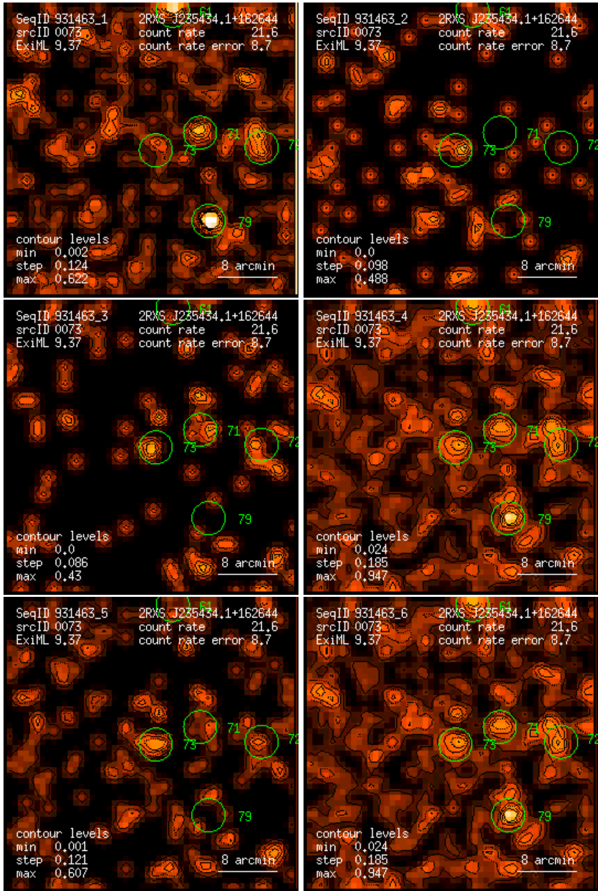
Figure 73: RASS 931463: detection 0073: band rate images, Gaussian filter: (1) PSPC channels 11 – 41, (2) 52 – 90, (3) 91 – 201, (4) 11 – 235, (5) 52 – 201, (6) 11 – 201. Broad band rates in counts/ks. Band rate contour levels in counts/ks/arcmin 2 .
