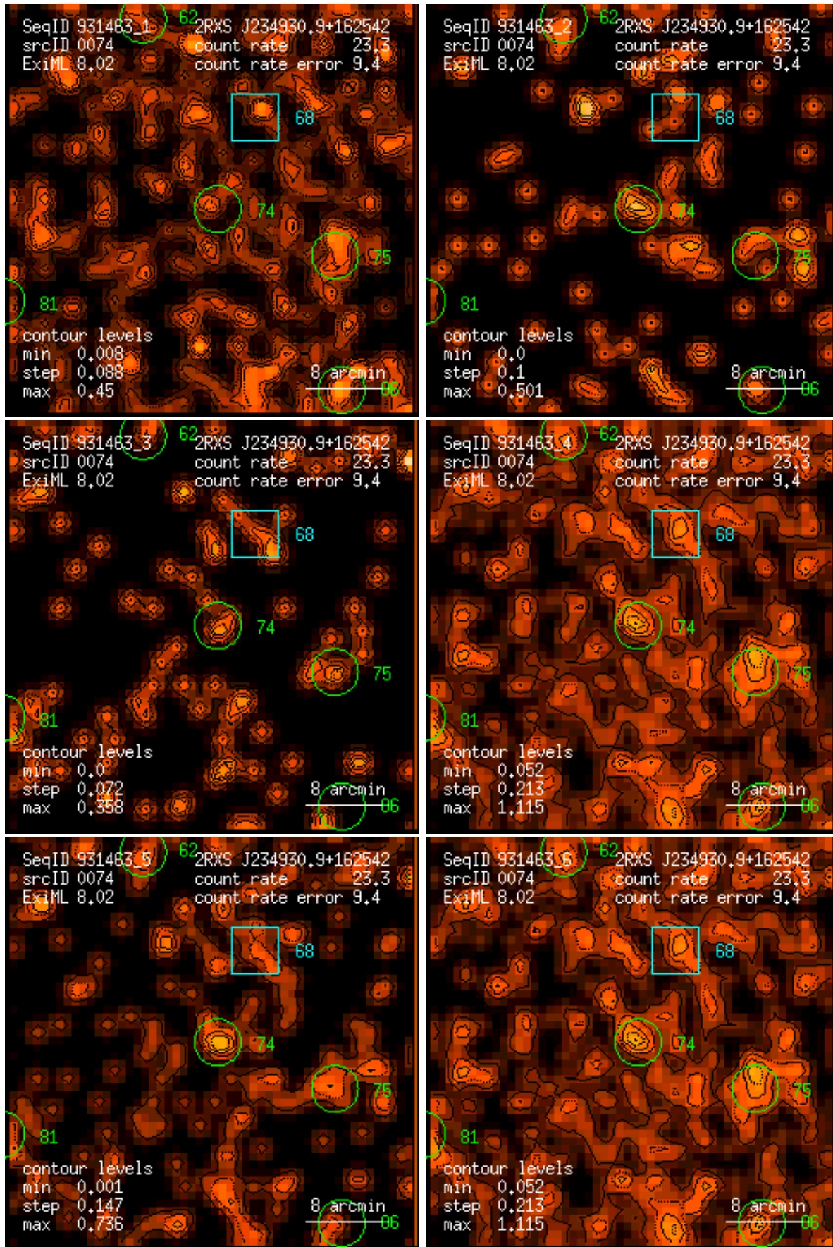
Figure 74: RASS 931463: detection 0074: band rate images, Gaussian filter: (1) PSPC channels 11 – 41, (2) 52 – 90, (3) 91 – 201, (4) 11 – 235, (5) 52 – 201, (6) 11 – 201. Broad band rates in counts/ks. Band rate contour levels in counts/ks/arcmin 2 .
