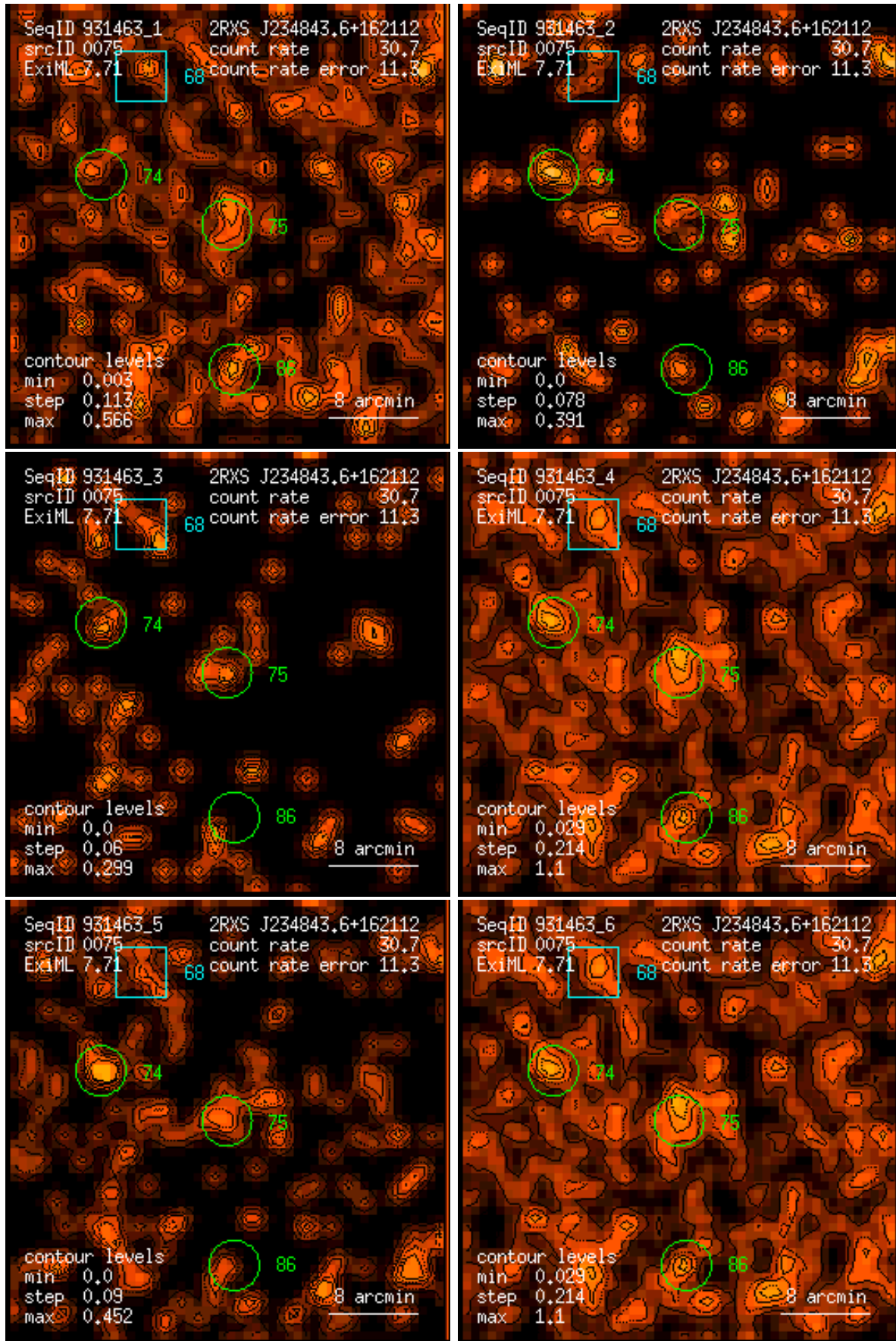
Figure 75: RASS 931463: detection 0075: band rate images, Gaussian filter: (1) PSPC channels 11 – 41, (2) 52 – 90, (3) 91 – 201, (4) 11 – 235, (5) 52 – 201, (6) 11 – 201. Broad band rates in counts/ks. Band rate contour levels in counts/ks/arcmin 2 .
