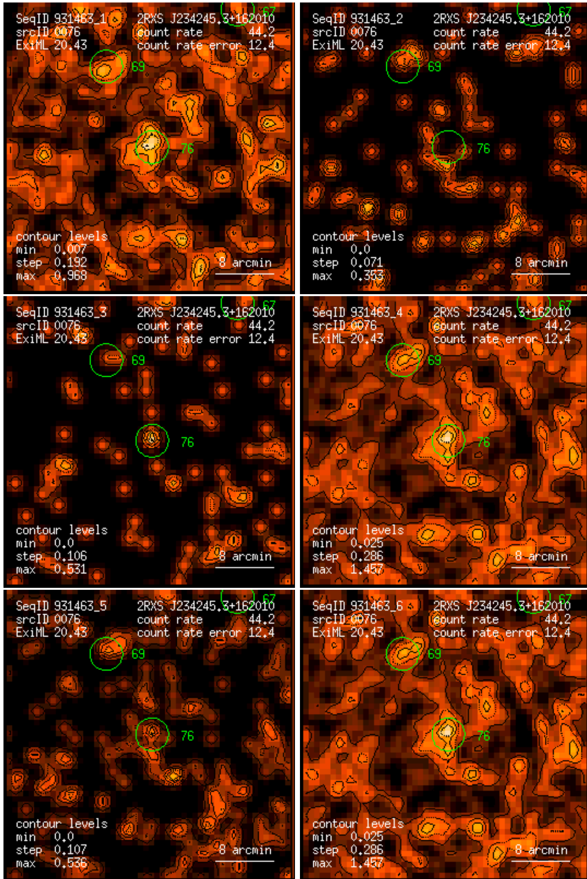
Figure 76: RASS 931463: detection 0076: band rate images, Gaussian filter: (1) PSPC channels 11 – 41, (2) 52 – 90, (3) 91 – 201, (4) 11 – 235, (5) 52 – 201, (6) 11 – 201. Broad band rates in counts/ks. Band rate contour levels in counts/ks/arcmin 2 .
