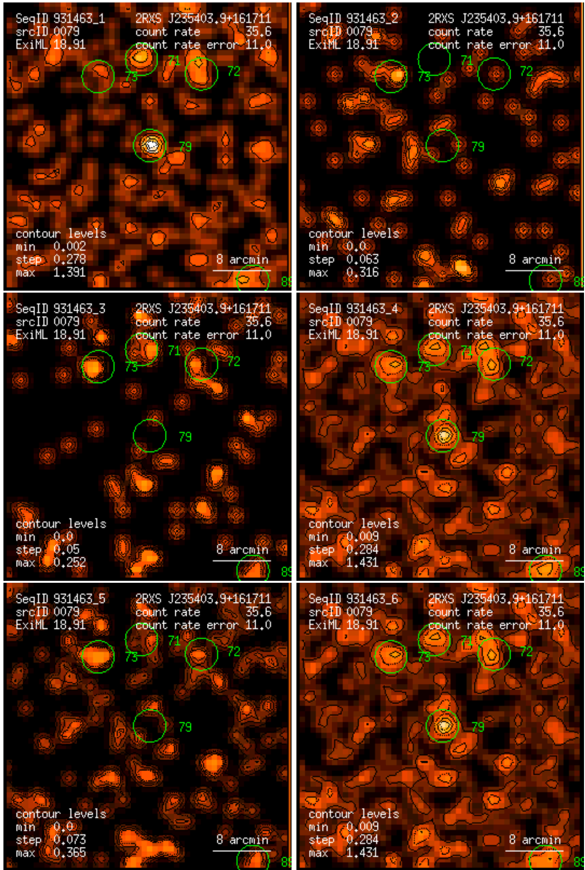
Figure 79: RASS 931463: detection 0079: band rate images, Gaussian filter: (1) PSPC channels 11 – 41, (2) 52 – 90, (3) 91 – 201, (4) 11 – 235, (5) 52 – 201, (6) 11 – 201. Broad band rates in counts/ks. Band rate contour levels in counts/ks/arcmin 2 .
