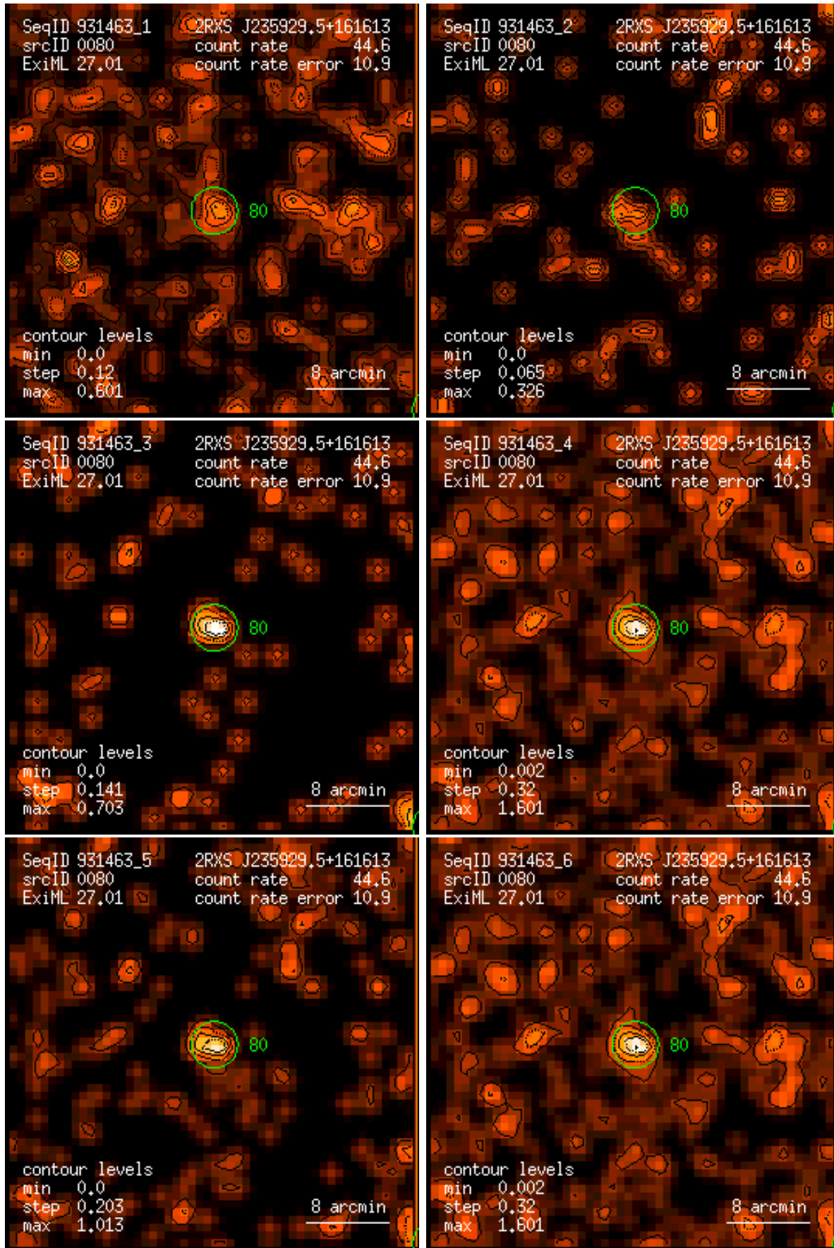
Figure 80: RASS 931463: detection 0080: band rate images, Gaussian filter: (1) PSPC channels 11 – 41, (2) 52 – 90, (3) 91 – 201, (4) 11 – 235, (5) 52 – 201, (6) 11 – 201. Broad band rates in counts/ks. Band rate contour levels in counts/ks/arcmin 2 .
