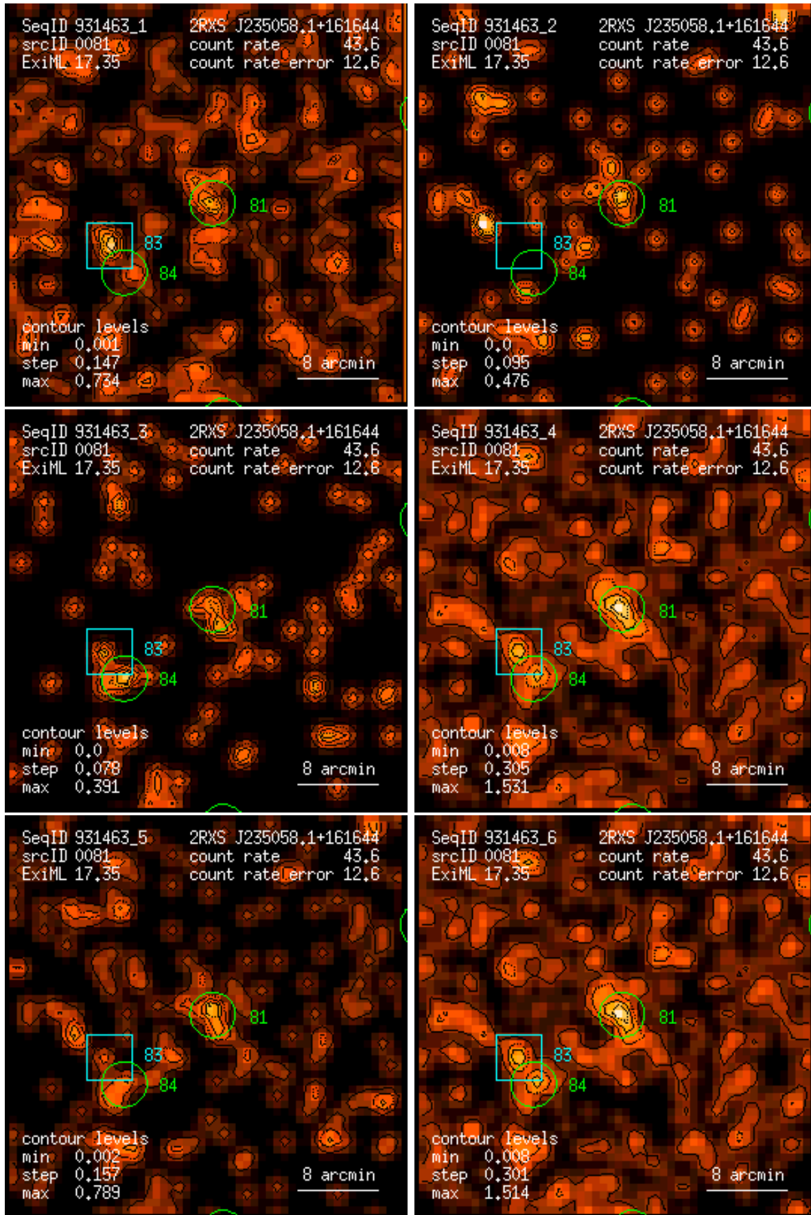
Figure 81: RASS 931463: detection 0081: band rate images, Gaussian filter: (1) PSPC channels 11 – 41, (2) 52 – 90, (3) 91 – 201, (4) 11 – 235, (5) 52 – 201, (6) 11 – 201. Broad band rates in counts/ks. Band rate contour levels in counts/ks/arcmin 2 .
