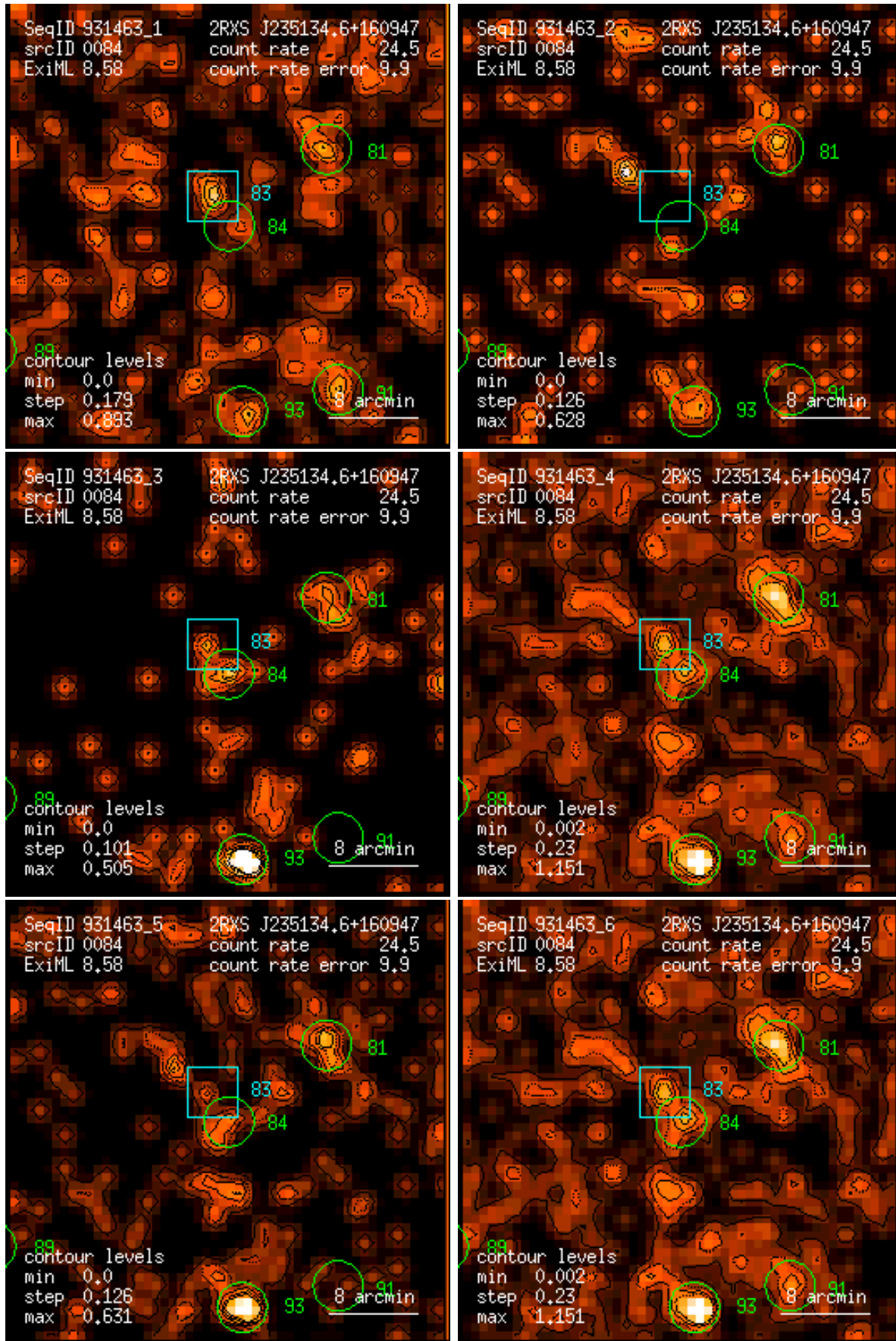
Figure 84: RASS 931463: detection 0084: band rate images, Gaussian filter: (1) PSPC channels 11 – 41, (2) 52 – 90, (3) 91 – 201, (4) 11 – 235, (5) 52 – 201, (6) 11 – 201. Broad band rates in counts/ks. Band rate contour levels in counts/ks/arcmin 2 .
