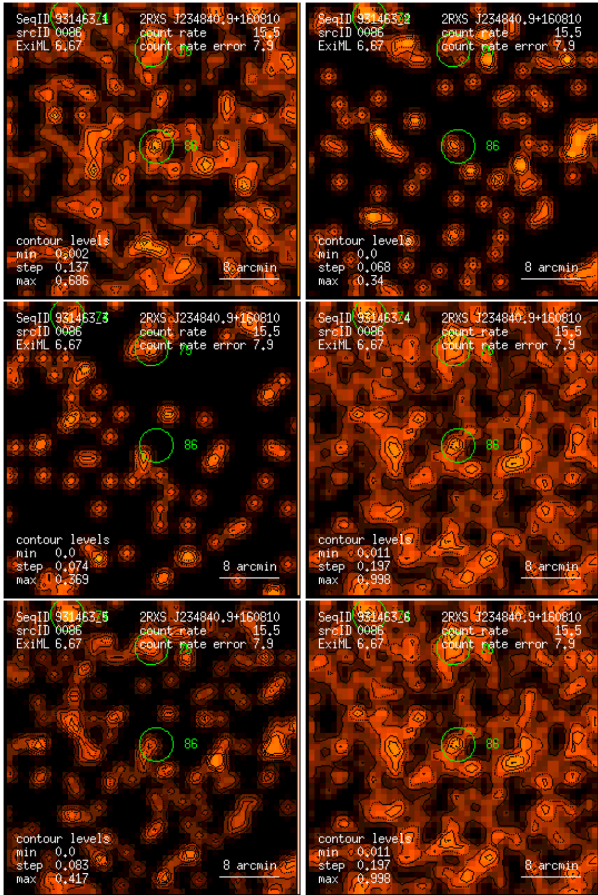
Figure 86: RASS 931463: detection 0086: band rate images, Gaussian filter: (1) PSPC channels 11 – 41, (2) 52 – 90, (3) 91 – 201, (4) 11 – 235, (5) 52 – 201, (6) 11 – 201. Broad band rates in counts/ks. Band rate contour levels in counts/ks/arcmin 2 .
