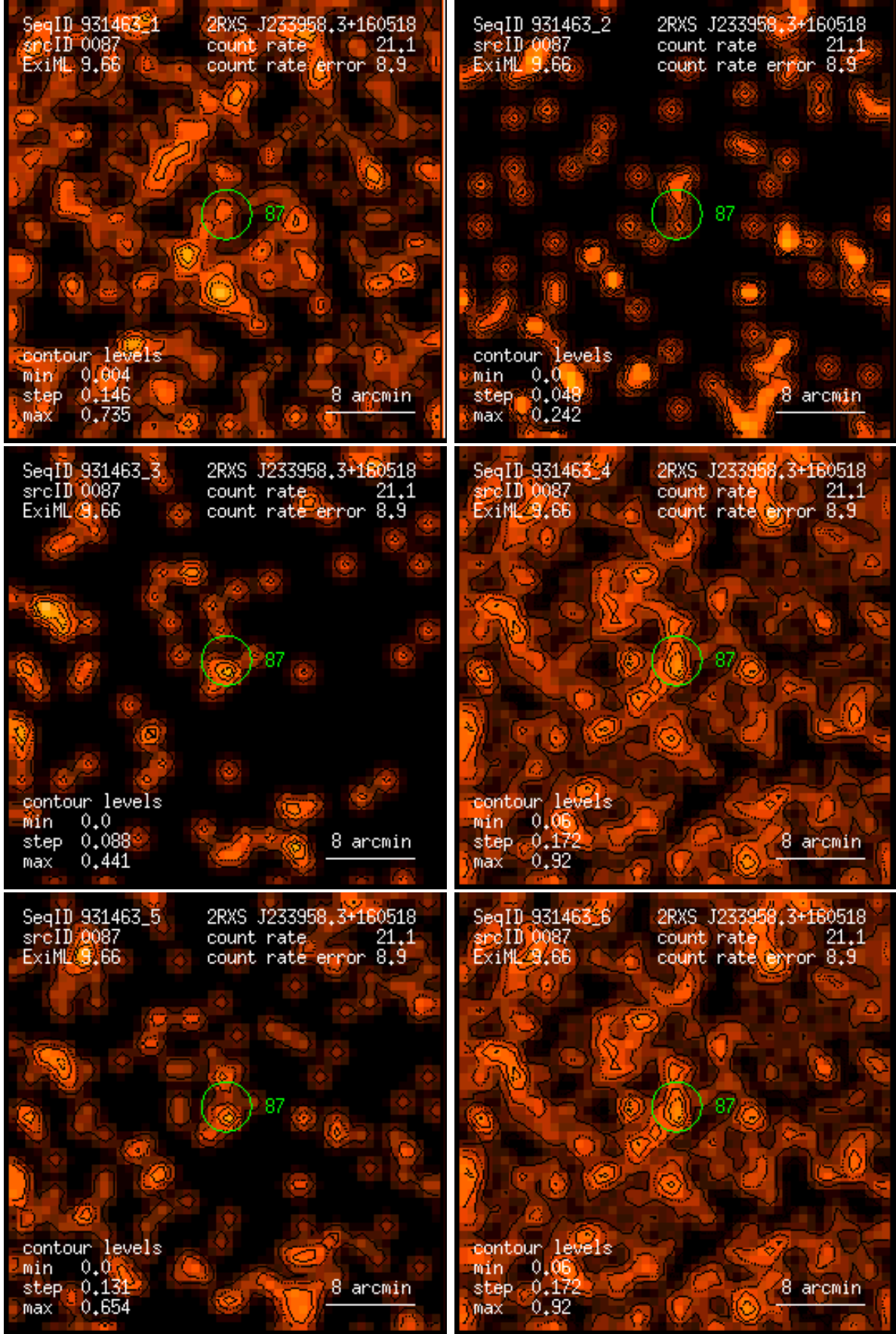
Figure 87: RASS 931463: detection 0087: band rate images, Gaussian filter: (1) PSPC channels 11 – 41, (2) 52 – 90, (3) 91 – 201, (4) 11 – 235, (5) 52 – 201, (6) 11 – 201. Broad band rates in counts/ks. Band rate contour levels in counts/ks/arcmin 2 .
