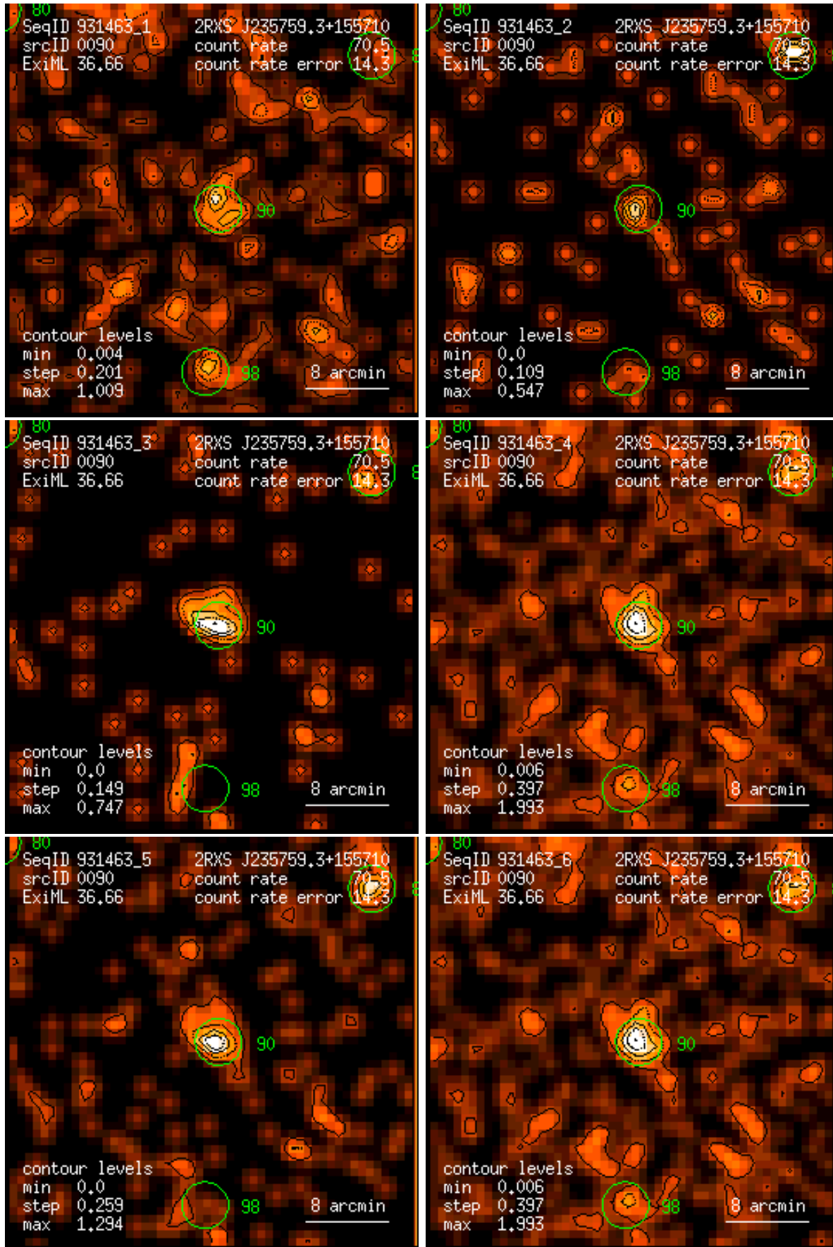
Figure 90: RASS 931463: detection 0090: band rate images, Gaussian filter: (1) PSPC channels 11 – 41, (2) 52 – 90, (3) 91 – 201, (4) 11 – 235, (5) 52 – 201, (6) 11 – 201. Broad band rates in counts/ks. Band rate contour levels in counts/ks/arcmin 2 .
