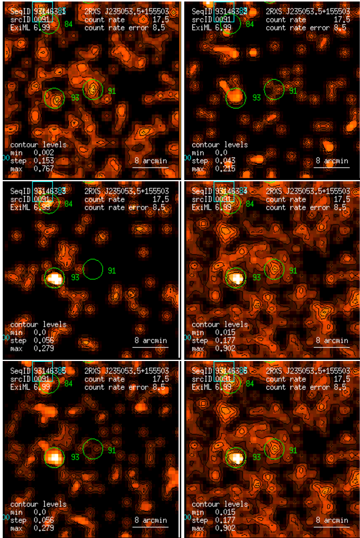
Figure 91: RASS 931463: detection 0091: band rate images, Gaussian filter: (1) PSPC channels 11 – 41, (2) 52 – 90, (3) 91 – 201, (4) 11 – 235, (5) 52 – 201, (6) 11 – 201. Broad band rates in counts/ks. Band rate contour levels in counts/ks/arcmin 2 .
