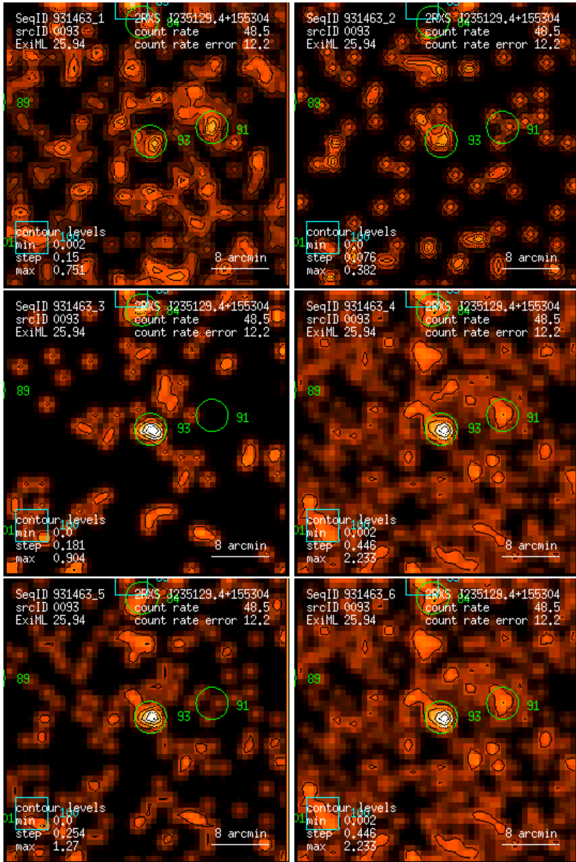
Figure 93: RASS 931463: detection 0093: band rate images, Gaussian filter: (1) PSPC channels 11 – 41, (2) 52 – 90, (3) 91 – 201, (4) 11 – 235, (5) 52 – 201, (6) 11 – 201. Broad band rates in counts/ks. Band rate contour levels in counts/ks/arcmin 2 .
