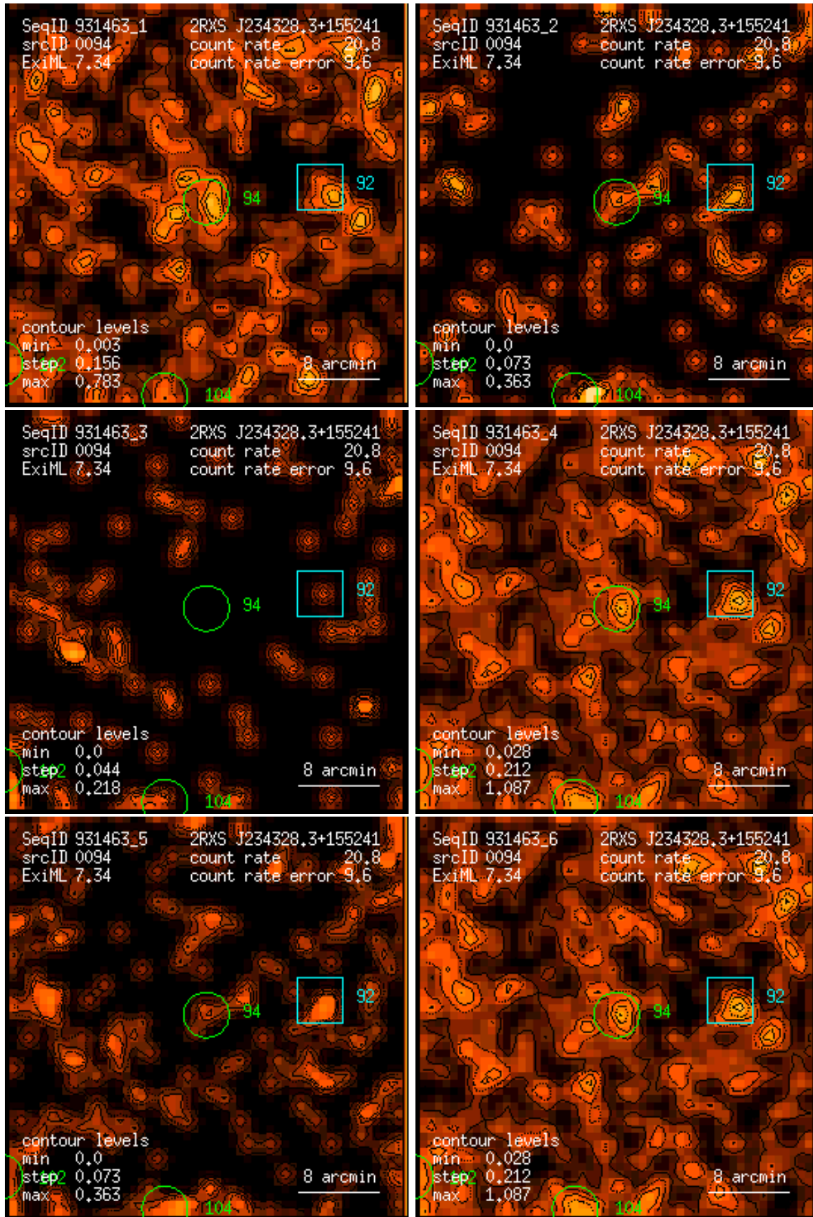
Figure 94: RASS 931463: detection 0094: band rate images, Gaussian filter: (1) PSPC channels 11 – 41, (2) 52 – 90, (3) 91 – 201, (4) 11 – 235, (5) 52 – 201, (6) 11 – 201. Broad band rates in counts/ks. Band rate contour levels in counts/ks/arcmin 2 .
