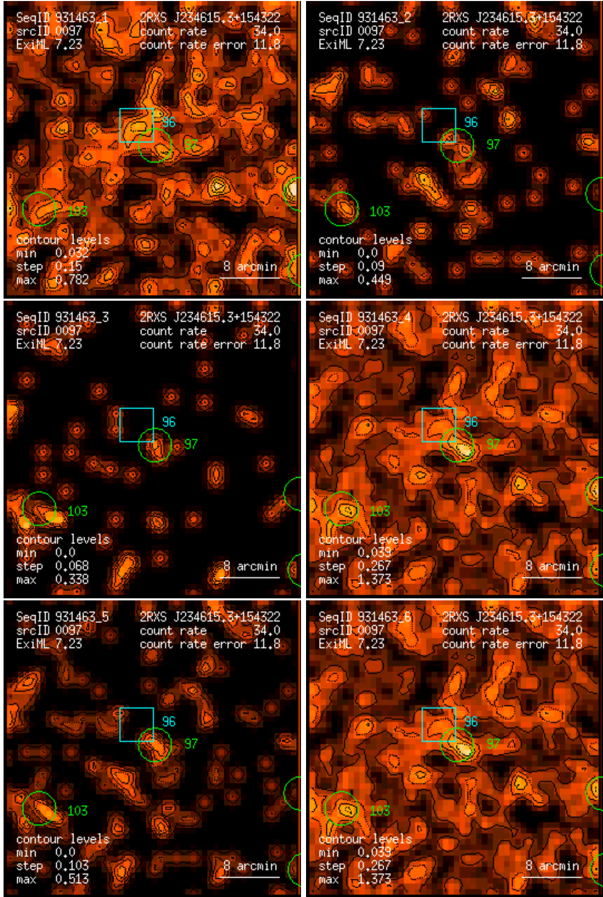
Figure 97: RASS 931463: detection 0097: band rate images, Gaussian filter: (1) PSPC channels 11 – 41, (2) 52 – 90, (3) 91 – 201, (4) 11 – 235, (5) 52 – 201, (6) 11 – 201. Broad band rates in counts/ks. Band rate contour levels in counts/ks/arcmin 2 .
