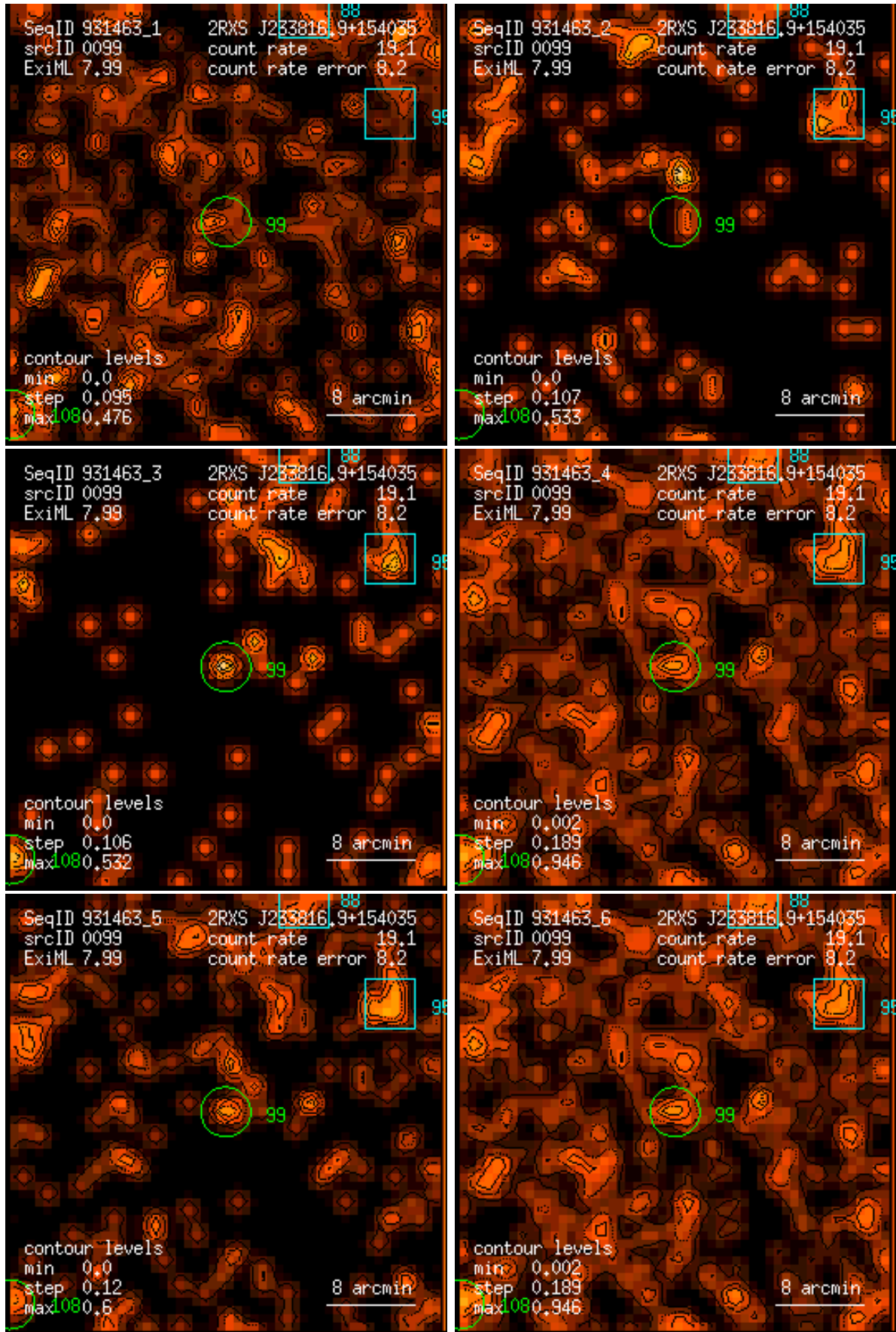
Figure 99: RASS 931463: detection 0099: band rate images, Gaussian filter: (1) PSPC channels 11 – 41, (2) 52 – 90, (3) 91 – 201, (4) 11 – 235, (5) 52 – 201, (6) 11 – 201. Broad band rates in counts/ks. Band rate contour levels in counts/ks/arcmin 2 .
