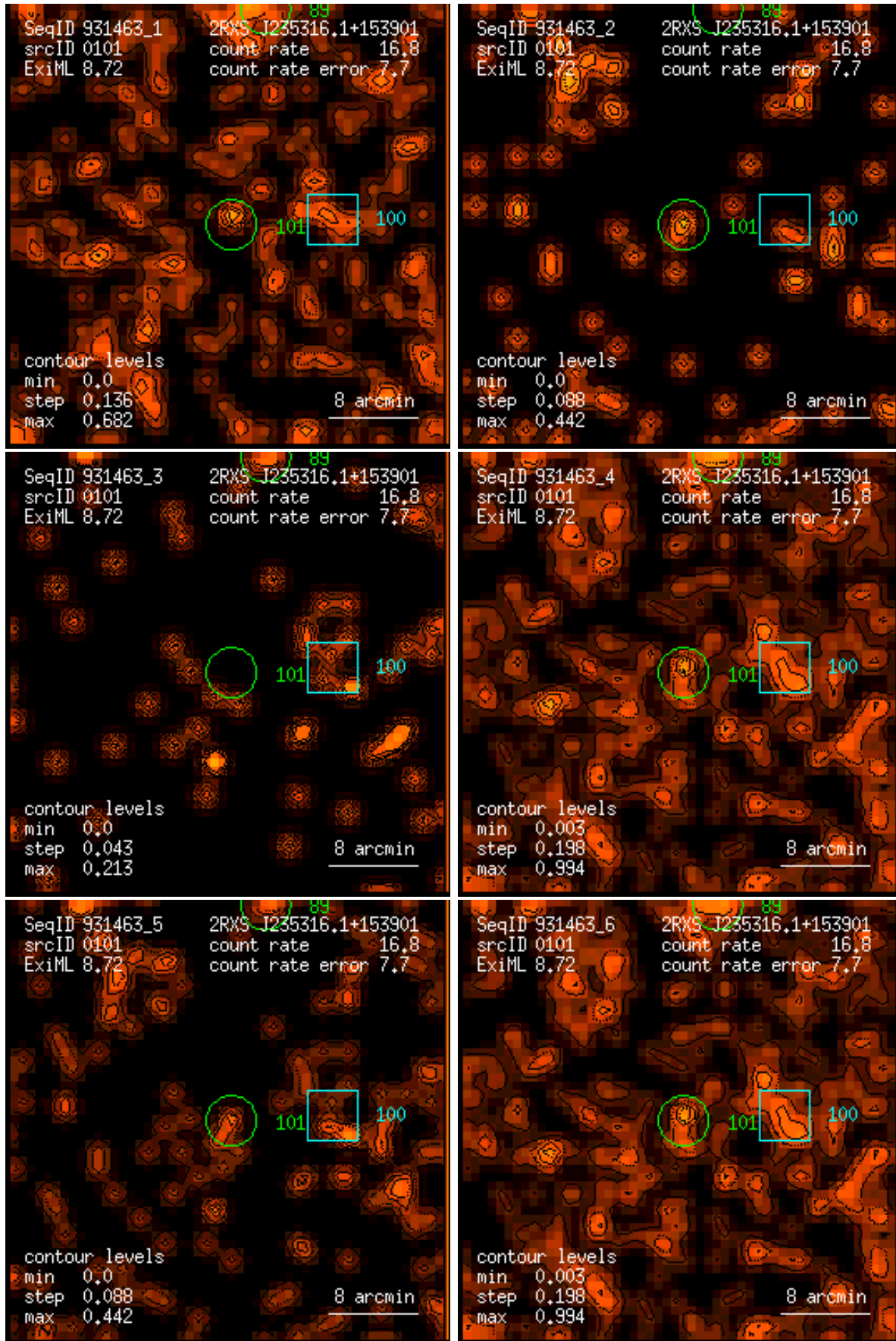
Figure 101: RASS 931463: detection 0101: band rate images, Gaussian filter: (1) PSPC channels 11 – 41, (2) 52 – 90, (3) 91 – 201, (4) 11 – 235, (5) 52 – 201, (6) 11 – 201. Broad band rates in counts/ks. Band rate contour levels in counts/ks/arcmin 2 .
