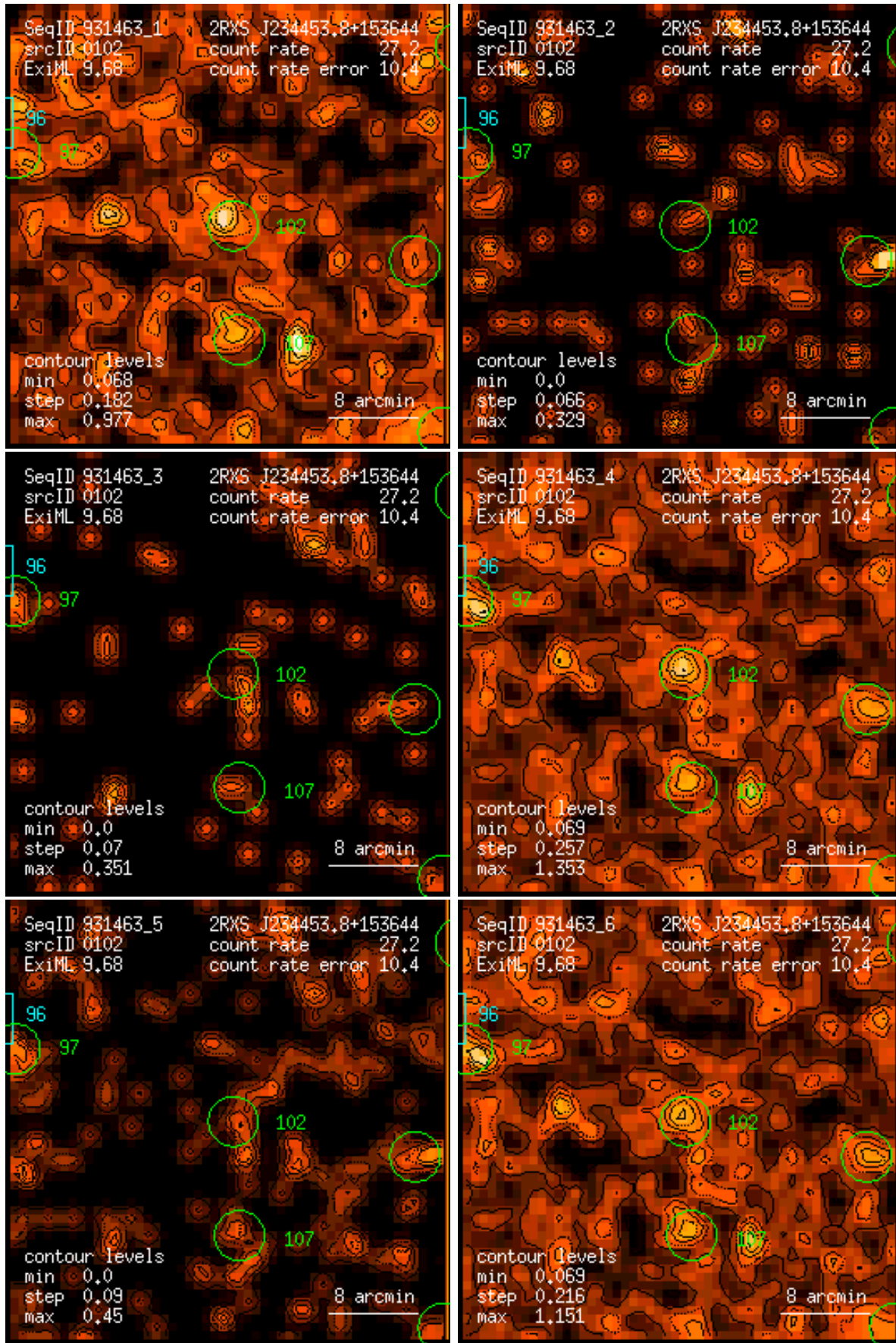
Figure 102: RASS 931463: detection 0102: band rate images, Gaussian filter: (1) PSPC channels 11 – 41, (2) 52 – 90, (3) 91 – 201, (4) 11 – 235, (5) 52 – 201, (6) 11 – 201. Broad band rates in counts/ks. Band rate contour levels in counts/ks/arcmin 2 .
