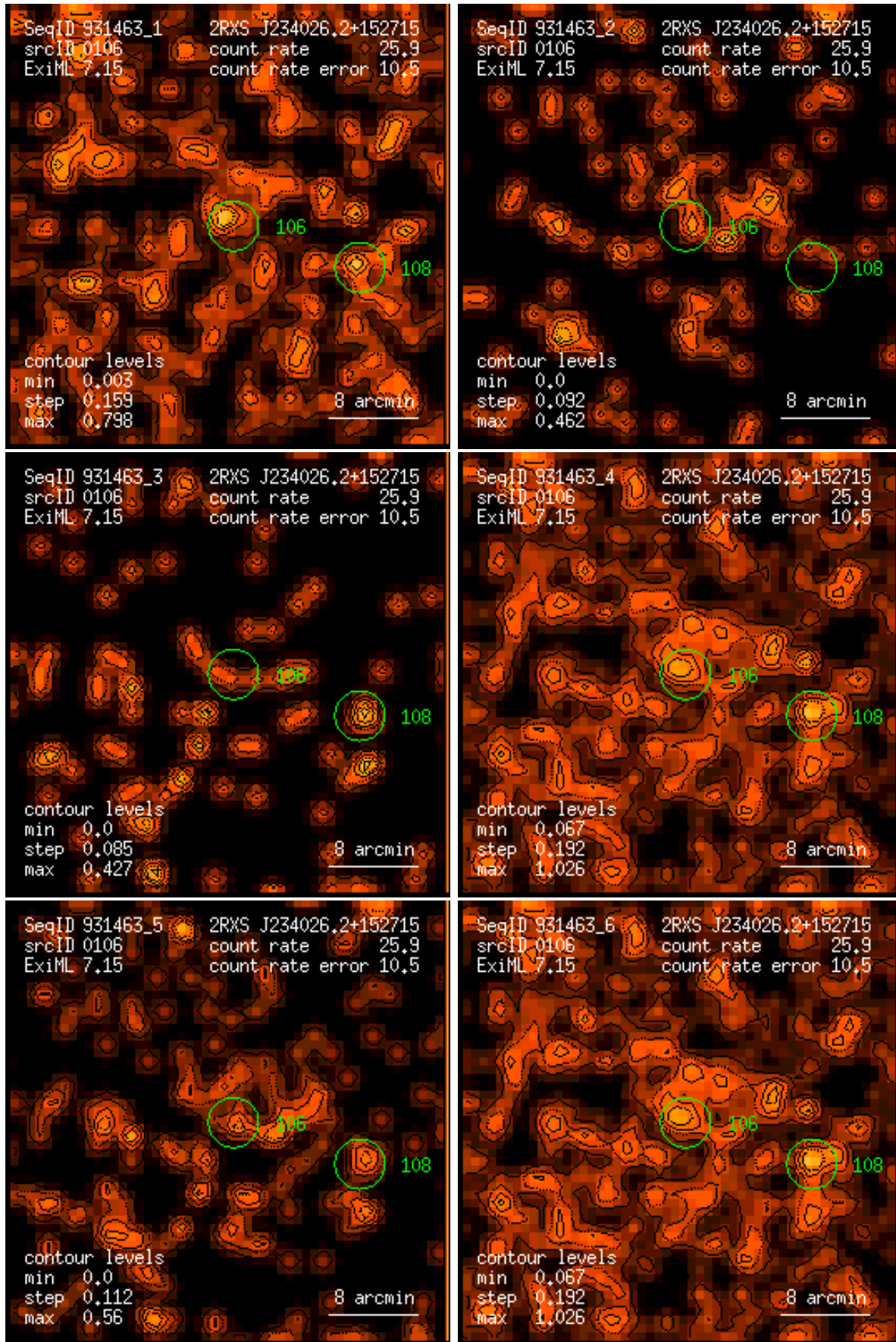
Figure 106: RASS 931463: detection 0106: band rate images, Gaussian filter: (1) PSPC channels 11 – 41, (2) 52 – 90, (3) 91 – 201, (4) 11 – 235, (5) 52 – 201, (6) 11 – 201. Broad band rates in counts/ks. Band rate contour levels in counts/ks/arcmin 2 .
