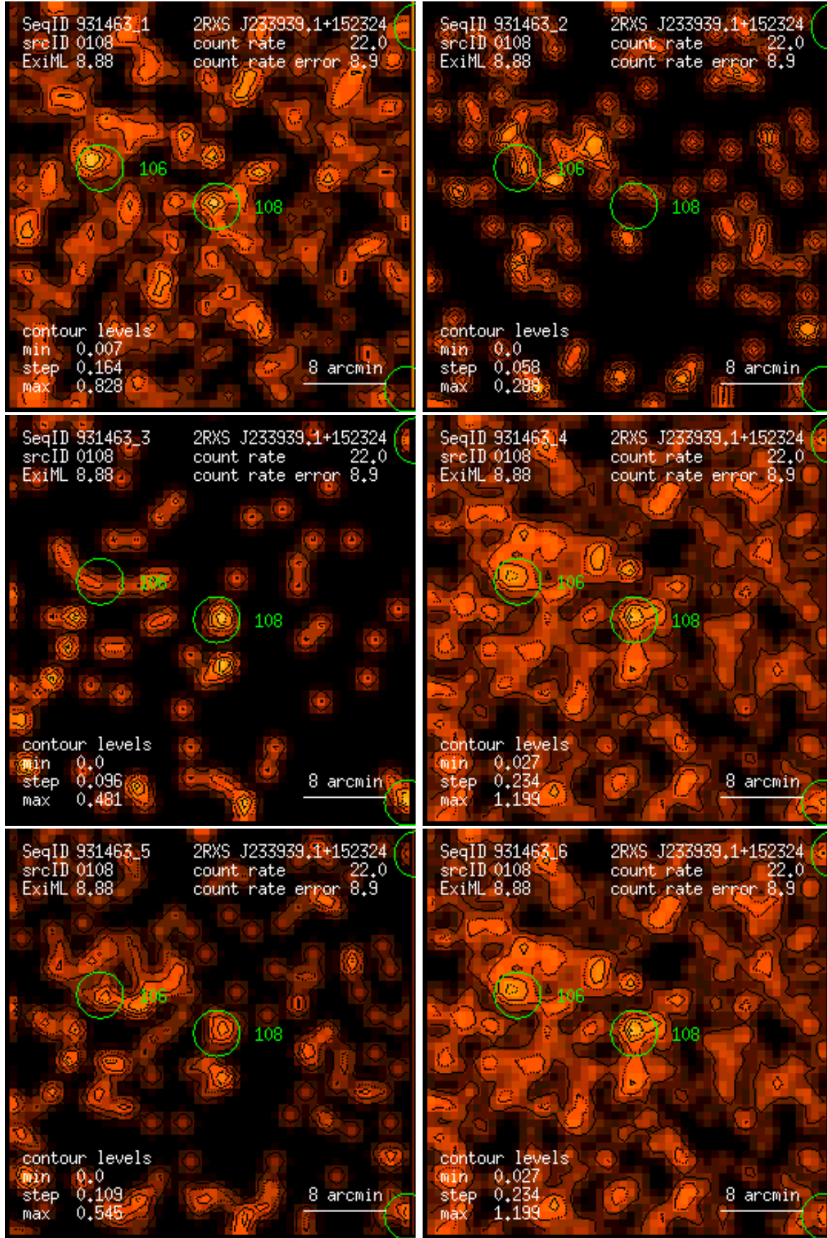
Figure 108: RASS 931463: detection 0108: band rate images, Gaussian filter: (1) PSPC channels 11 – 41, (2) 52 – 90, (3) 91 – 201, (4) 11 – 235, (5) 52 – 201, (6) 11 – 201. Broad band rates in counts/ks. Band rate contour levels in counts/ks/arcmin 2 .
