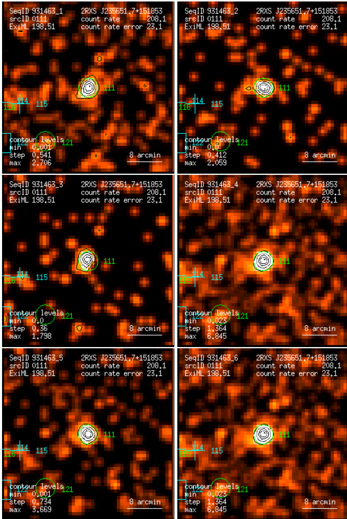
Figure 111: RASS 931463: detection 0111: band rate images, Gaussian filter: (1) PSPC channels 11 – 41, (2) 52 – 90, (3) 91 – 201, (4) 11 – 235, (5) 52 – 201, (6) 11 – 201. Broad band rates in counts/ks. Band rate contour levels in counts/ks/arcmin 2 .
