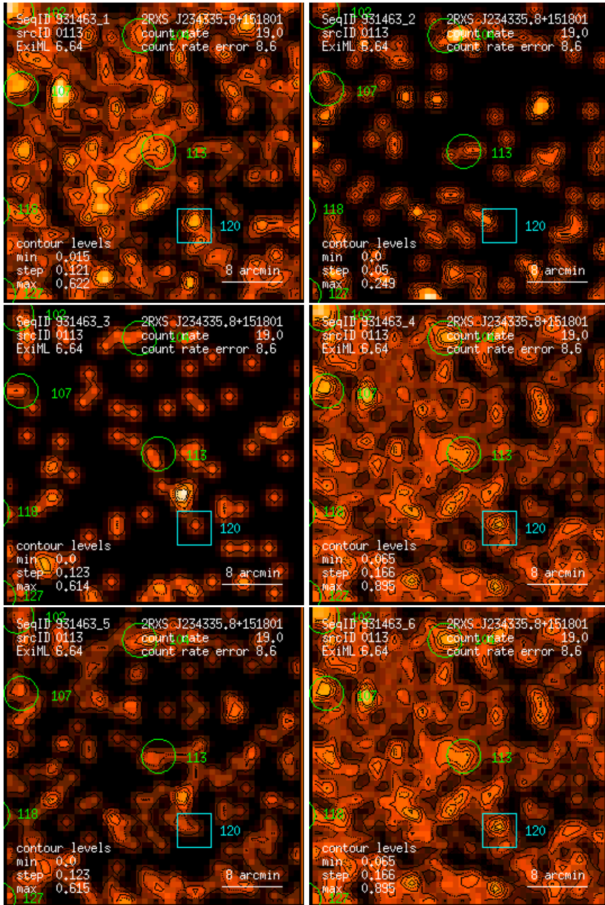
Figure 113: RASS 931463: detection 0113: band rate images, Gaussian filter: (1) PSPC channels 11 – 41, (2) 52 – 90, (3) 91 – 201, (4) 11 – 235, (5) 52 – 201, (6) 11 – 201. Broad band rates in counts/ks. Band rate contour levels in counts/ks/arcmin 2 .
