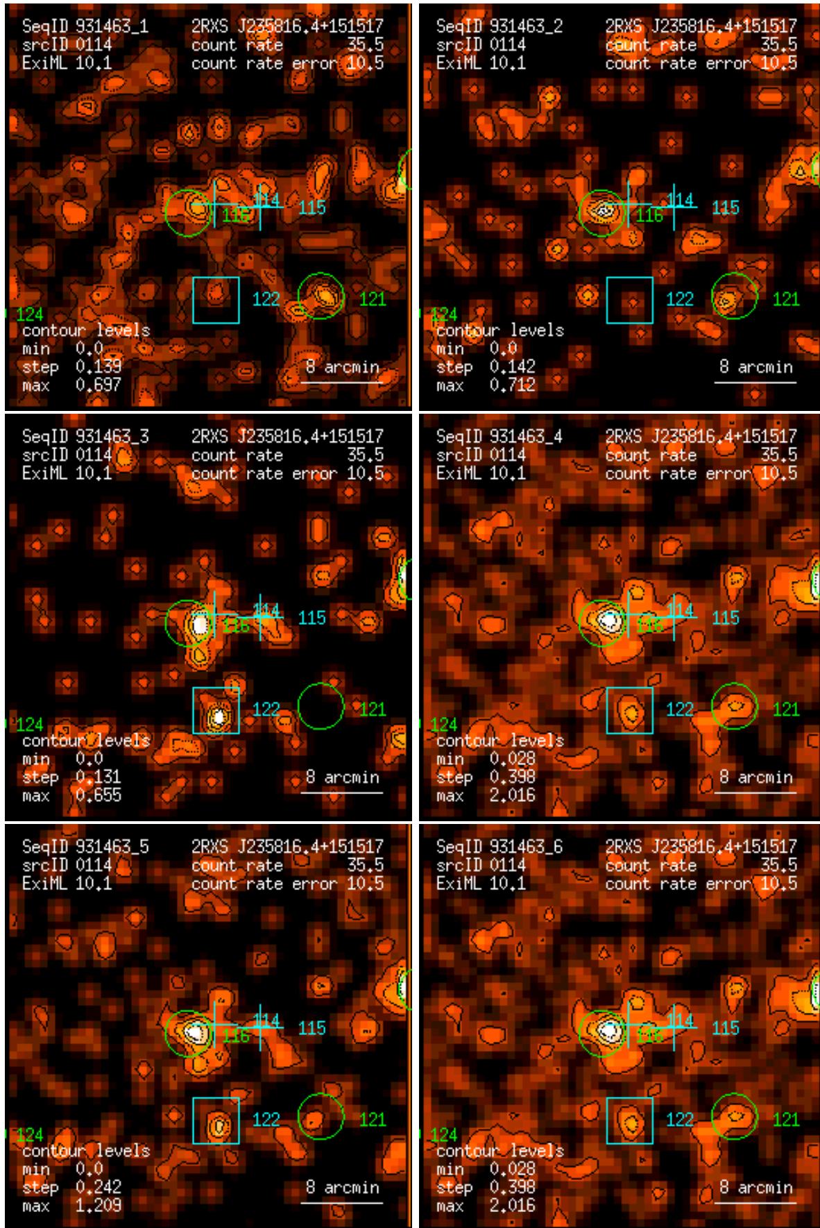
Figure 114: RASS 931463: detection 0114: band rate images, Gaussian filter: (1) PSPC channels 11 – 41, (2) 52 – 90, (3) 91 – 201, (4) 11 – 235, (5) 52 – 201, (6) 11 – 201. Broad band rates in counts/ks. Band rate contour levels in counts/ks/arcmin 2 .
