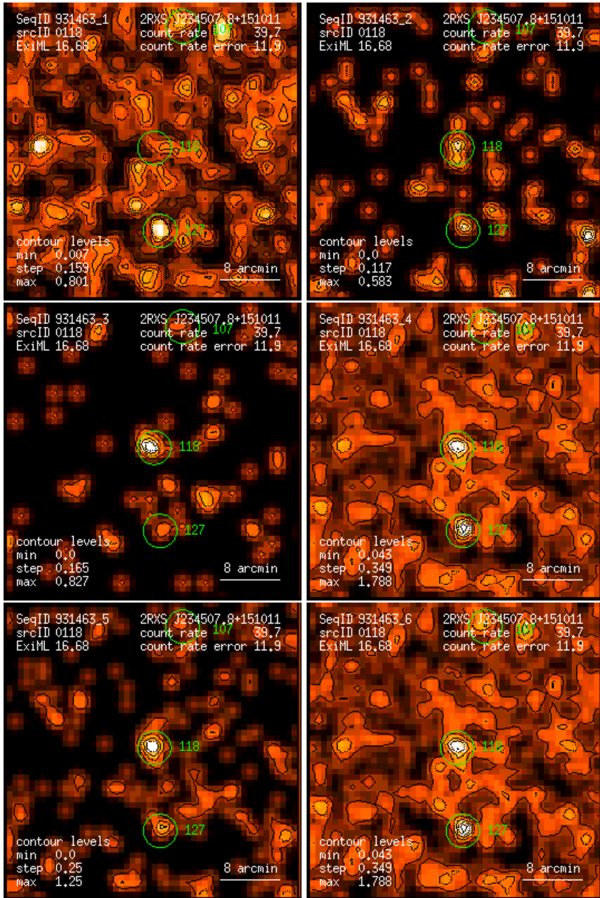
Figure 118: RASS 931463: detection 0118: band rate images, Gaussian filter: (1) PSPC channels 11 – 41, (2) 52 – 90, (3) 91 – 201, (4) 11 – 235, (5) 52 – 201, (6) 11 – 201. Broad band rates in counts/ks. Band rate contour levels in counts/ks/arcmin 2 .
