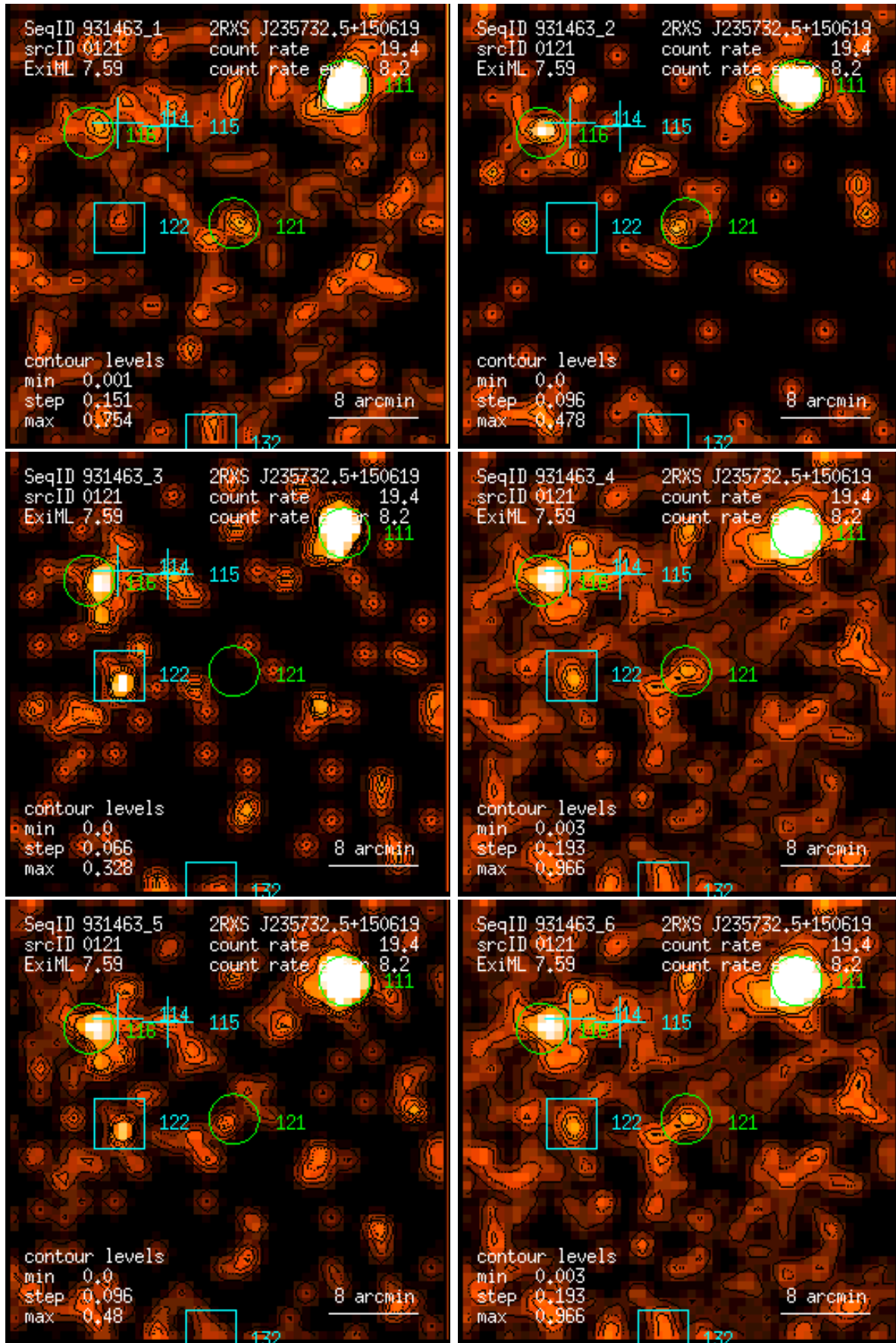
Figure 121: RASS 931463: detection 0121: band rate images, Gaussian filter: (1) PSPC channels 11 – 41, (2) 52 – 90, (3) 91 – 201, (4) 11 – 235, (5) 52 – 201, (6) 11 – 201. Broad band rates in counts/ks. Band rate contour levels in counts/ks/arcmin 2 .
