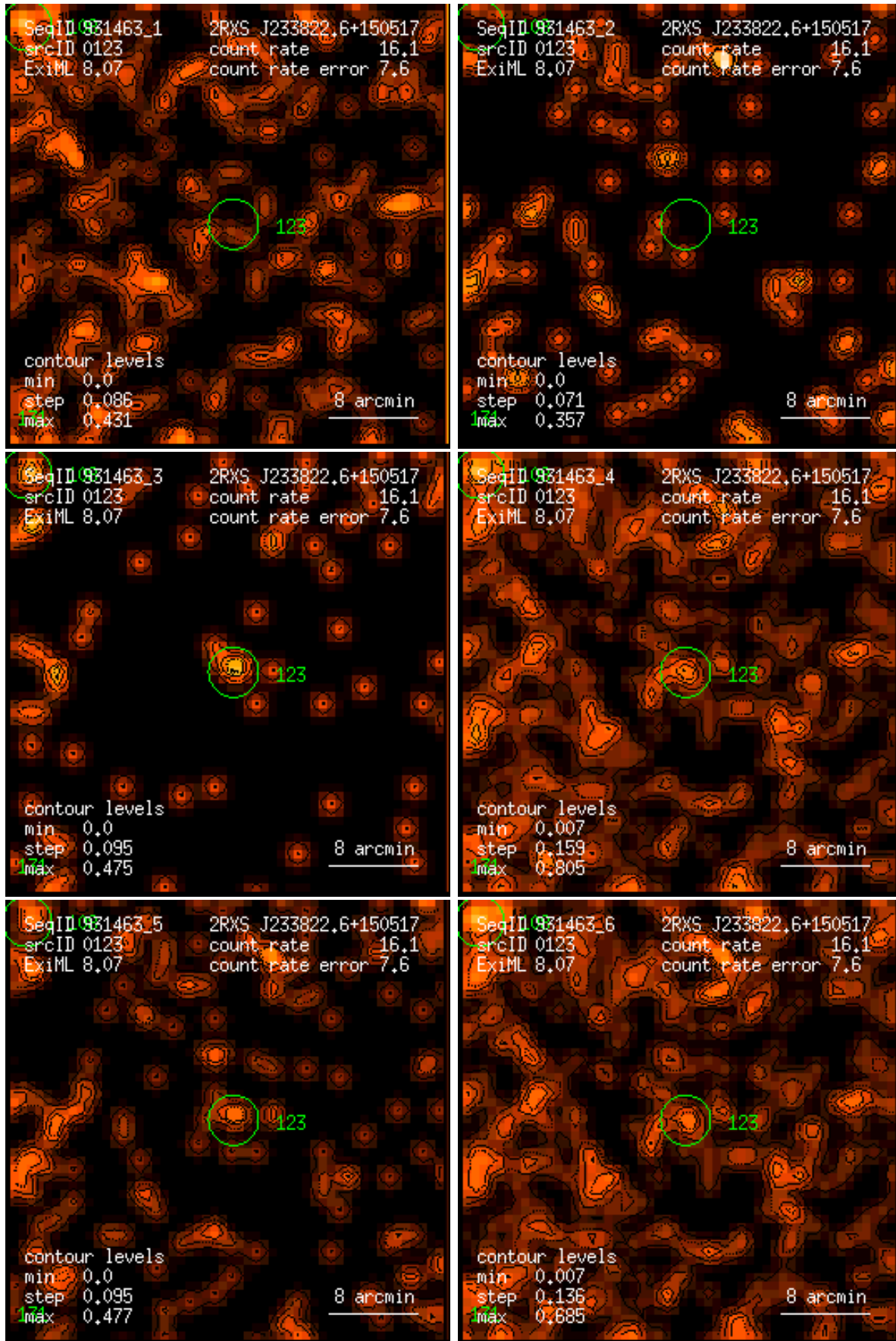
Figure 123: RASS 931463: detection 0123: band rate images, Gaussian filter: (1) PSPC channels 11 – 41, (2) 52 – 90, (3) 91 – 201, (4) 11 – 235, (5) 52 – 201, (6) 11 – 201. Broad band rates in counts/ks. Band rate contour levels in counts/ks/arcmin 2 .
