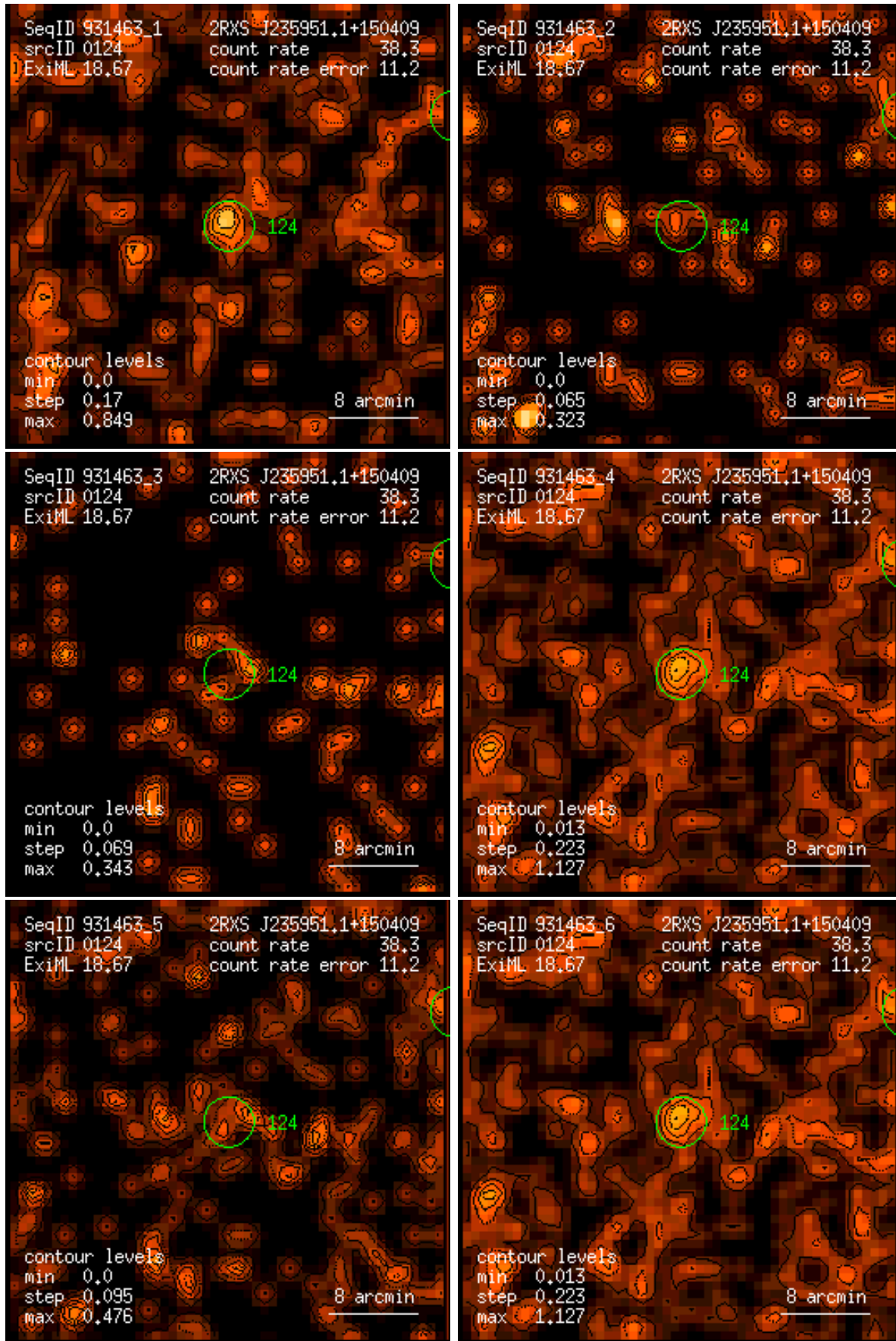
Figure 124: RASS 931463: detection 0124: band rate images, Gaussian filter: (1) PSPC channels 11 – 41, (2) 52 – 90, (3) 91 – 201, (4) 11 – 235, (5) 52 – 201, (6) 11 – 201. Broad band rates in counts/ks. Band rate contour levels in counts/ks/arcmin 2 .
