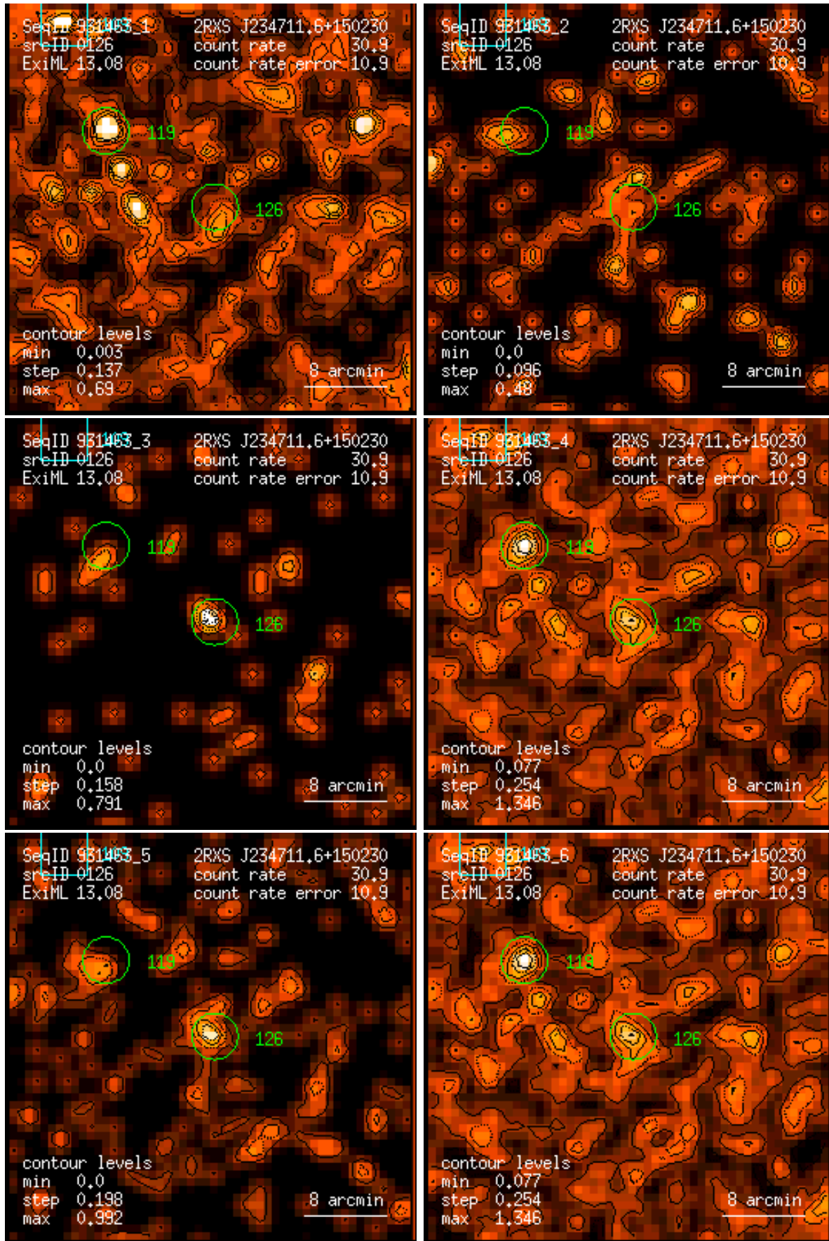
Figure 126: RASS 931463: detection 0126: band rate images, Gaussian filter: (1) PSPC channels 11 – 41, (2) 52 – 90, (3) 91 – 201, (4) 11 – 235, (5) 52 – 201, (6) 11 – 201. Broad band rates in counts/ks. Band rate contour levels in counts/ks/arcmin 2 .
