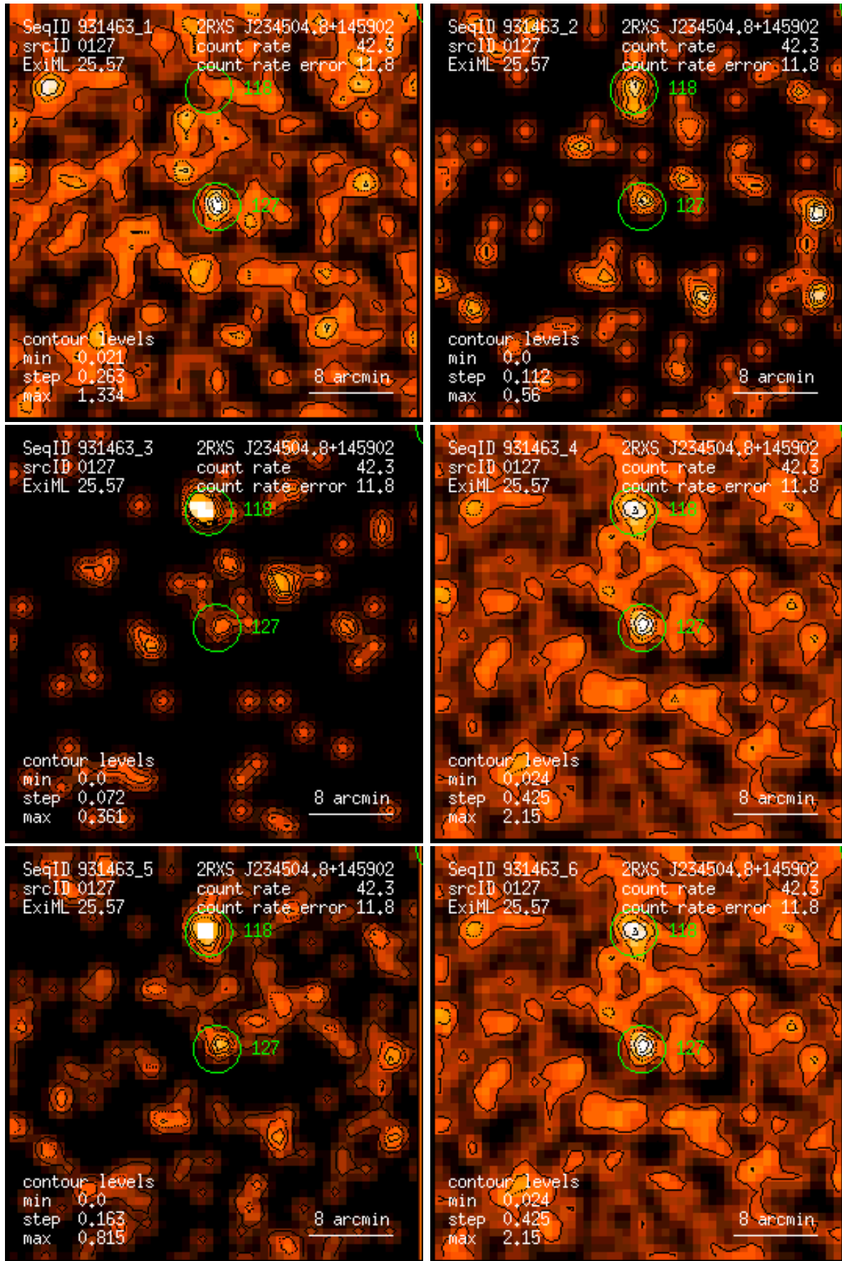
Figure 127: RASS 931463: detection 0127: band rate images, Gaussian filter: (1) PSPC channels 11 – 41, (2) 52 – 90, (3) 91 – 201, (4) 11 – 235, (5) 52 – 201, (6) 11 – 201. Broad band rates in counts/ks. Band rate contour levels in counts/ks/arcmin 2 .
